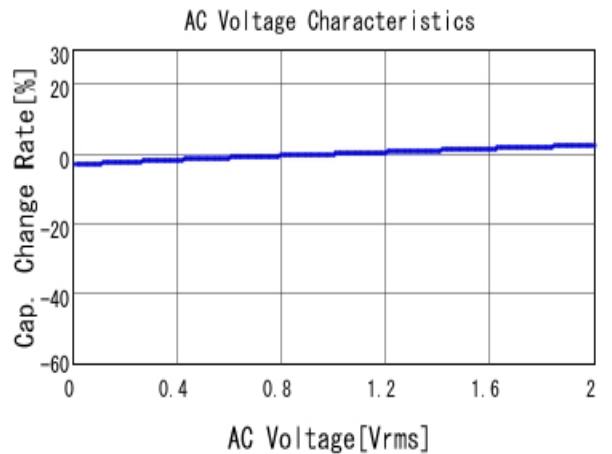
■ GCJ31CR72A105KA01 C-AC Voltage capchange, DCOV, 25.0d
