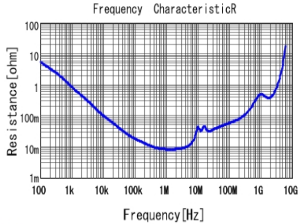
■ GCJ31CR72A105KA01 R DCOV, 25degC
