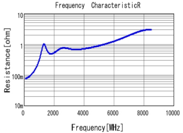
■ GCM1885C2A331JA16 R DC0V, 25degC
