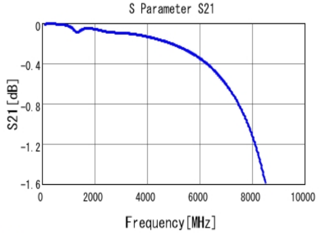
■ GCM1885C2A331JA16 S21 DCOV, 25degC
