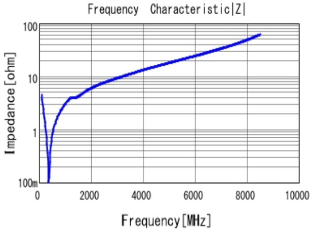
■ GCM1885C2A331JA16 |Z| DC0V, 25degC
