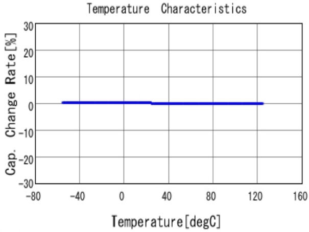
■ GCM1885C2A331JA16 C-Temp. capchange, DCOV, AC1Vrms
