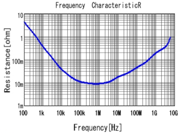
■ GRT155C80J475ME13 R DCOV, 25degC
