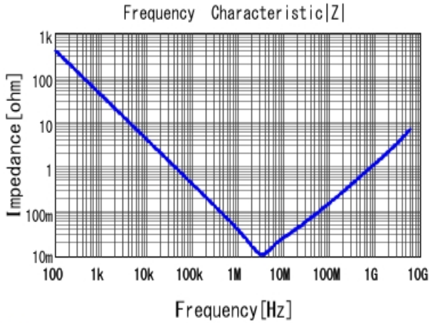
■ GRT155C80J475ME13 |Z| DCOV, 25degC
