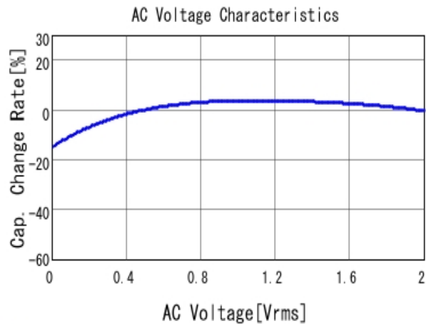
■ GRT155C80J475ME13 C-AC Voltage capchange, DCOV, 25.0d
