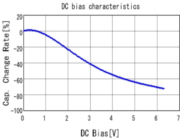
■ GRT155C80J475ME13 C-DC bias capchange, 25.0degC, AC0.
