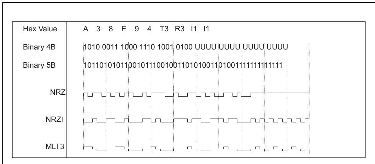
FIGURE 9-1: MLT3 CODING
