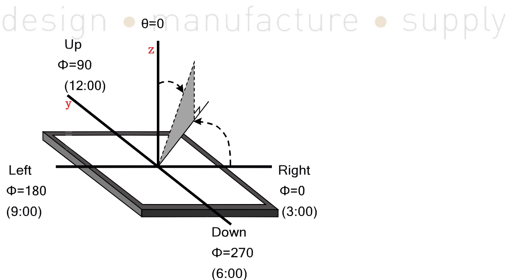
FIG.3.The definition of viewing angle
