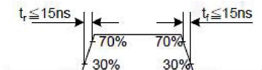
Display Serial Interface Timing Characteristics (3-line SPI system)
