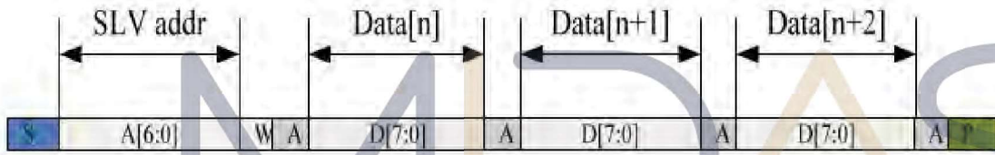
Figure 2-5 I2C master write, slave read
