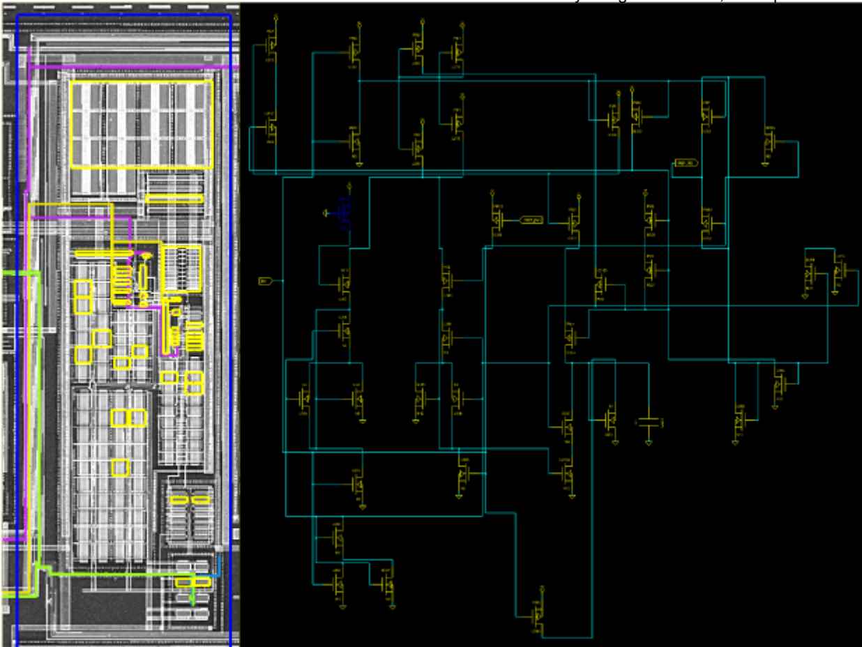
Figure 1. These images from the third-party reverse-engineering study of the DS28E38 show the layout and schematic of the circuit.
