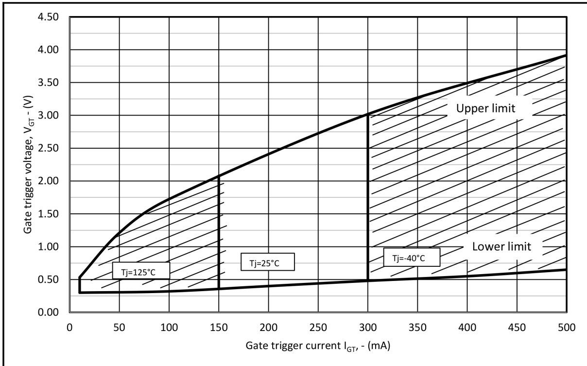
Fig.12 Gate characteristics
