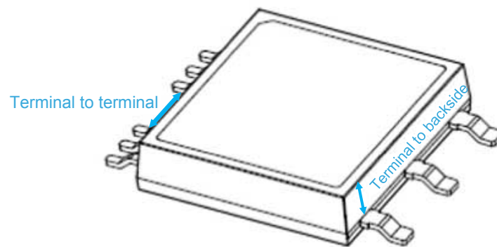
Figure 15. Creepage distance measurement
