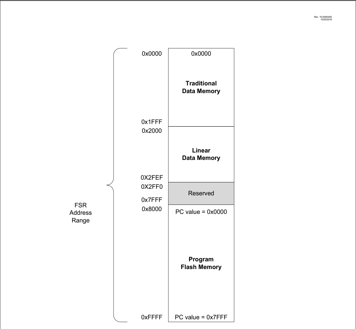
FIGURE 3-8: INDIRECT ADDRESSING
