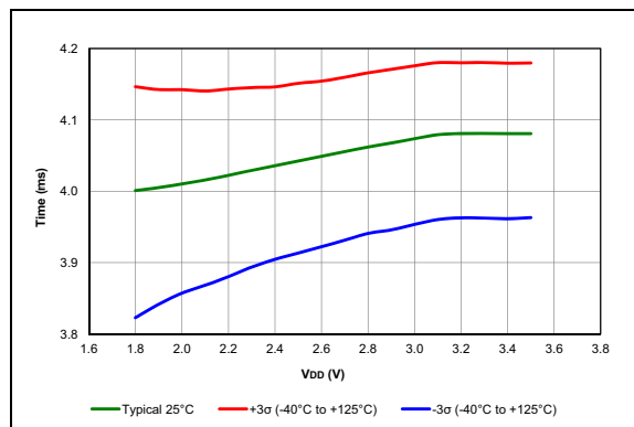
FIGURE 38-10: WDT Time-Out Period, PIC16LF18857/77 Only.
