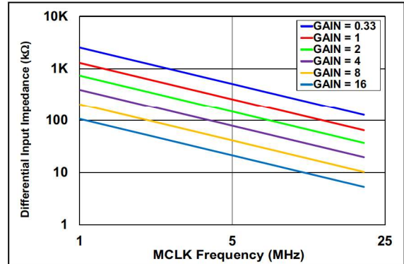
FIGURE 2-52: Differential Input Impedance vs. MCLK .
