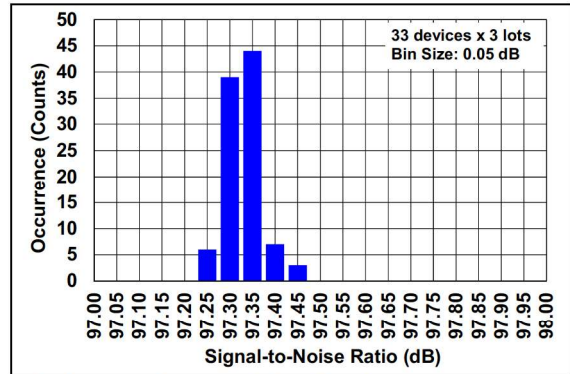
FIGURE 2-18: SNR Distribution Histogram.
