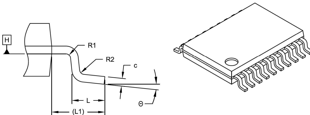
DETAIL B
