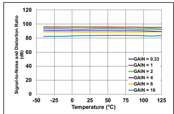
FIGURE 2-30: SINAD vs. Temperature, Internal V_{REF} .
