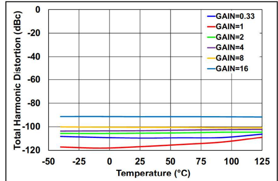
FIGURE 2-28: THD vs. Temperature.
