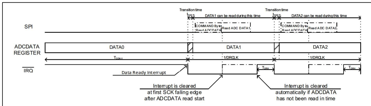
FIGURE 6-13: Data Ready Interrupt \overline{IRQ} Pin Timing Diagram.
