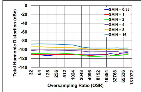
FIGURE 2-16: SFDR vs. OSR.
