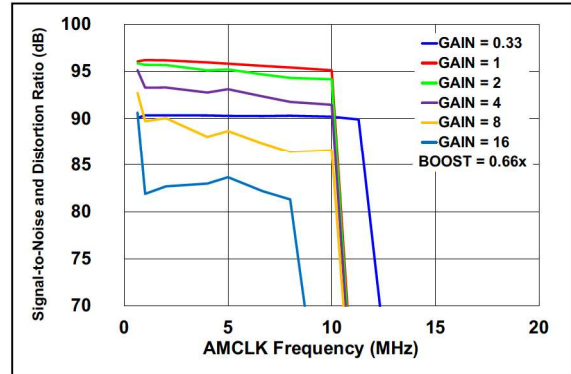
FIGURE 2-40: SINAD vs. AMCLK (Boost = 0.66x, Internal V_{REF} ).
