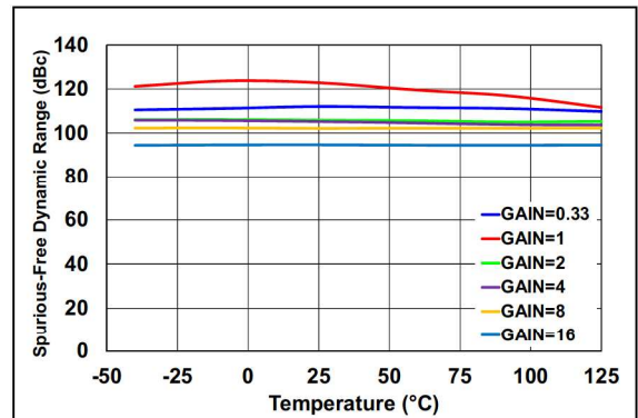
FIGURE 2-29: SFDR vs. Temperature.
