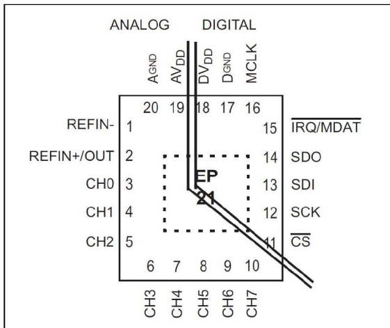
FIGURE 7-7: Separation of Analog and Digital Circuits on the Layout (Shown on the UQFN Package).
