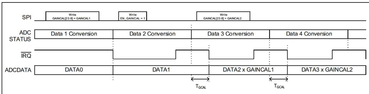
FIGURE 5-13: ADC Output and \overline{IRQ} Behavior with Digital Gain Error Calibration Enabled.
