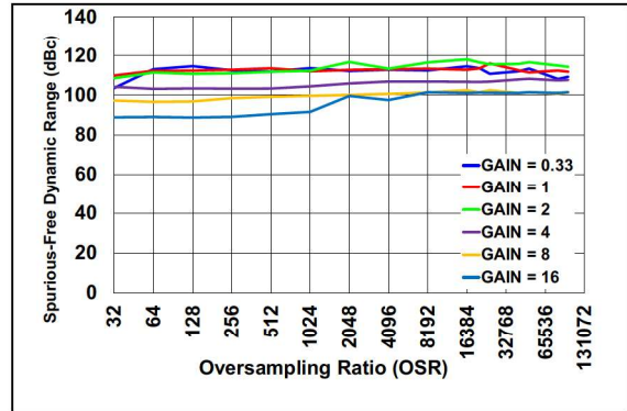
FIGURE 2-17: SFDR vs. OSR, Internal V_{REF} .
