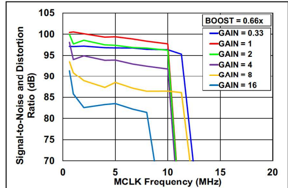
FIGURE 2-40: SINAD vs. MCLK (BOOST = 0.66x, Internal V_{REF} ).
