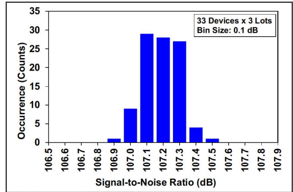
FIGURE 2-18: SNR Distribution Histogram External V_{REF} .
