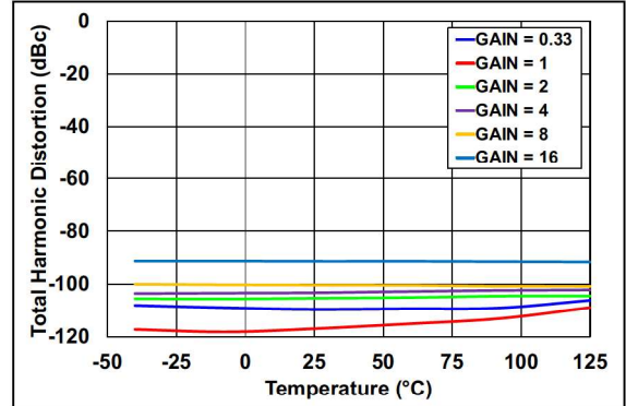
FIGURE 2-28: THD vs. Temperature, External V_{REF} .
