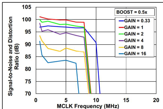
FIGURE 2-39: SINAD vs. MCLK (BOOST = 0.5x, Internal V_{REF} ).
