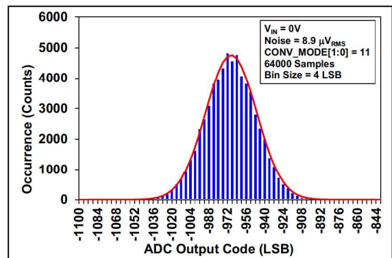
FIGURE 2-5: Output Noise Histogram (External V_{REF} ).
