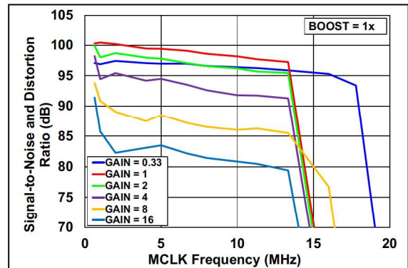
FIGURE 2-41: SINAD vs. MCLK (BOOST = 1x, Internal V_{REF} ).
