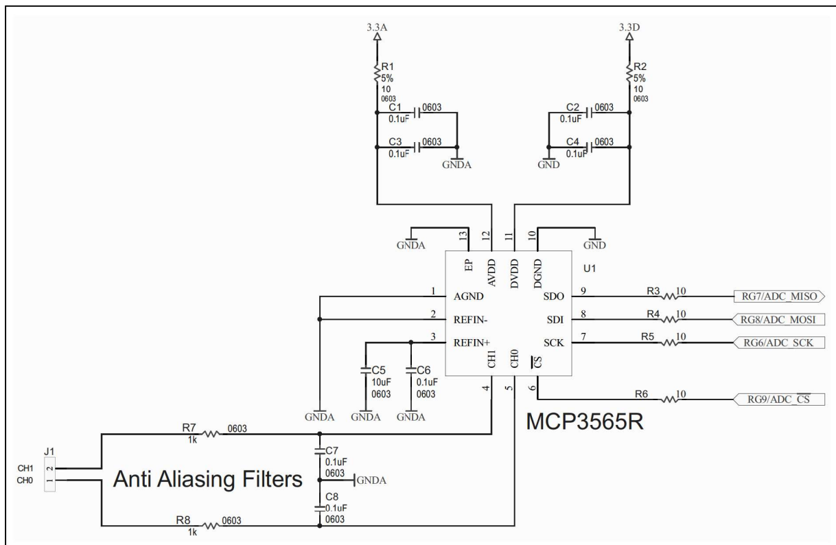
FIGURE 7-1: MCP3565R Application Example.
