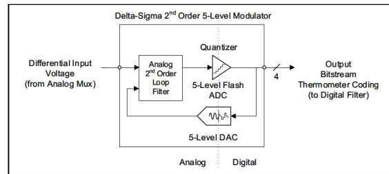
FIGURE 5-2: Simplified Delta-Sigma ADC Block Diagram.
