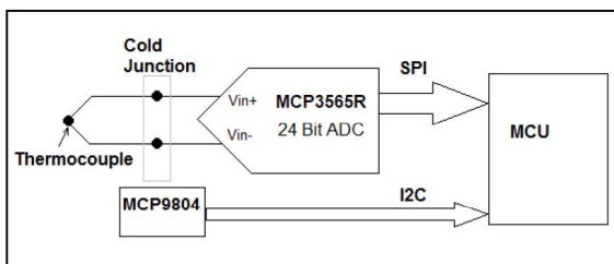
FIGURE 7-2: Thermocouple Connection.
