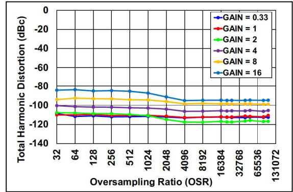
FIGURE 2-16: THD vs. OSR Internal V_{REF} .
