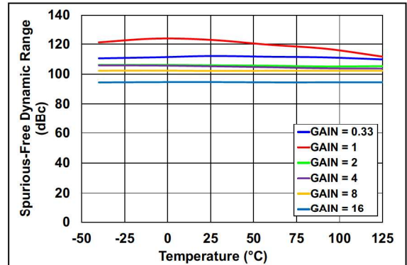
FIGURE 2-29: SFDR vs. Temperature, External V_{REF} .
