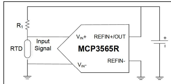
FIGURE 7-3: Wheatstone Bridge Ratiometric Connection.
