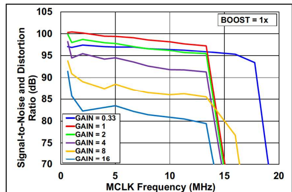
FIGURE 2-42: SINAD vs. MCLK (BOOST = 2x, Internal V_{REF} ).
