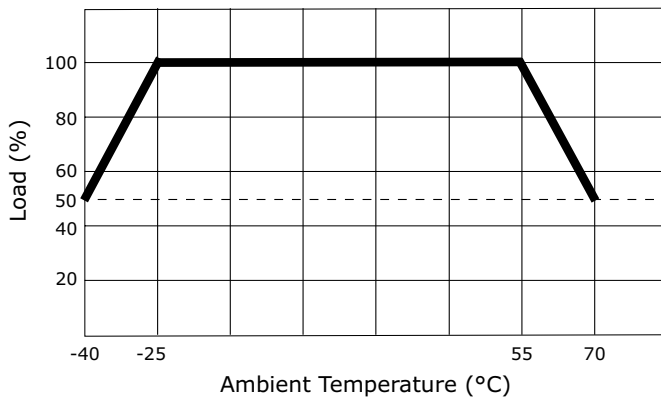
Load vs. Ambient Temperature (at 85~305 Vac / 120~430 Vdc Input Voltage)
