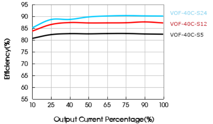
Efficiency vs. Load Current (at 230 Vac)
