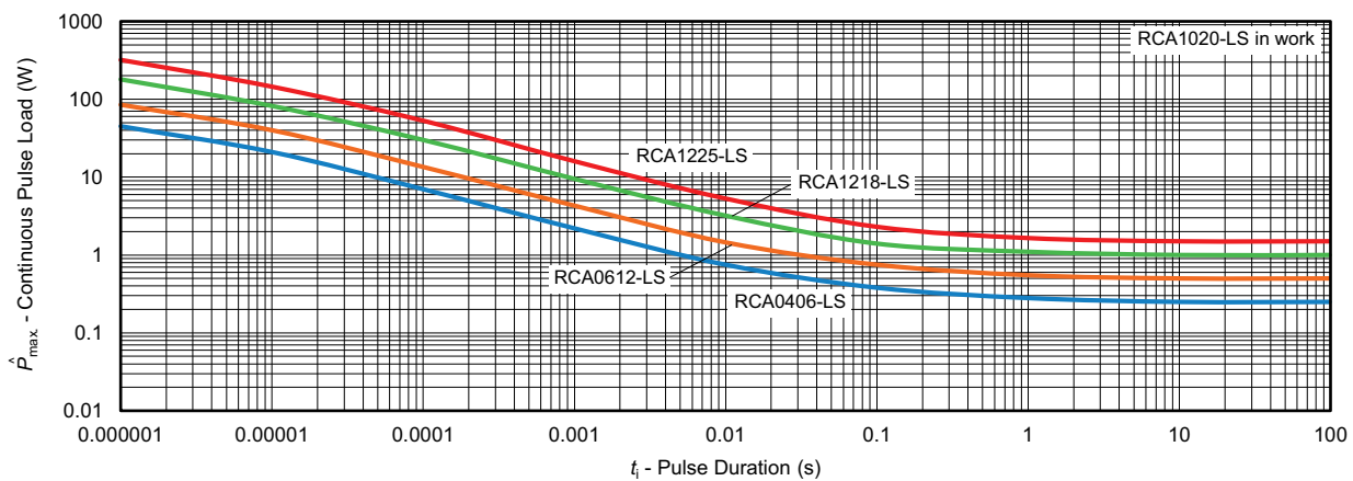
Maximum pulse load, continuous pulses; applicable if \bar{P} \leq P(g_{amb}) and \hat{U} \leq \hat{U}_{max} ; for permissible resistance change equivalent to 8000 h operation
