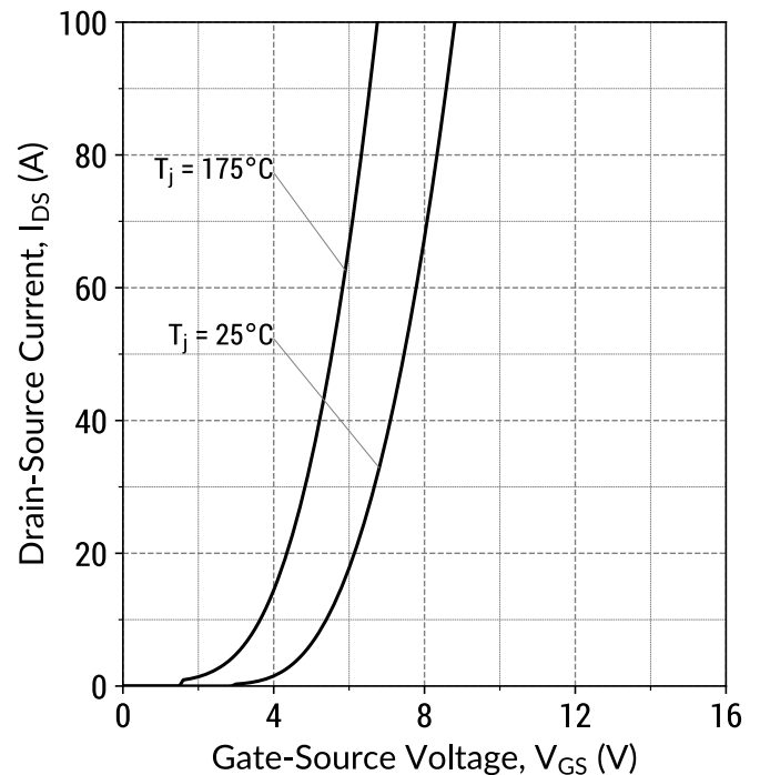
Figure 4: Transfer Characteristics ( V_{DS} = 10\text{ V} )
