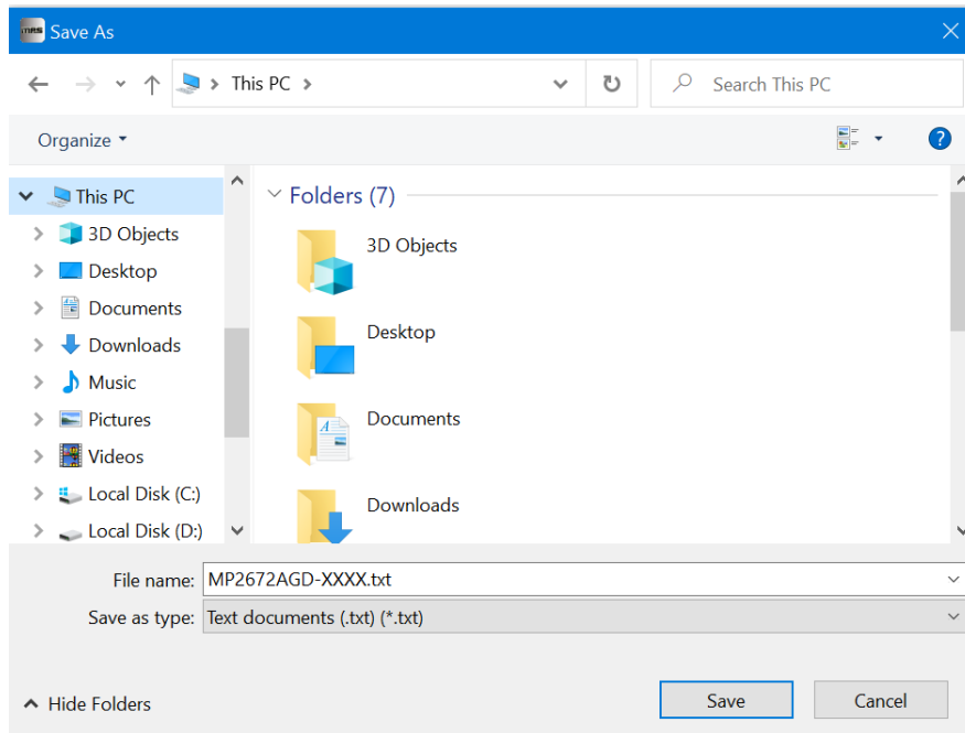
Figure 11: Saving Configurations
