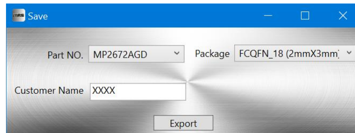
Figure 10: Exporting Configurations
