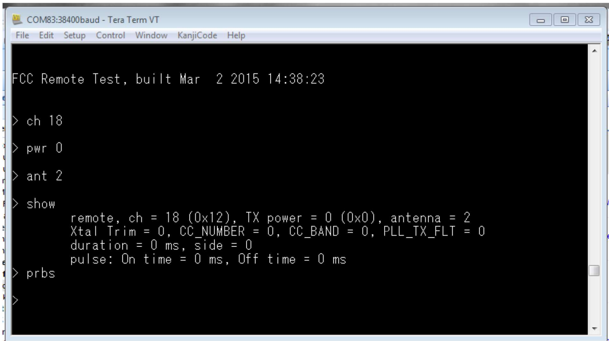
Figure 3-2. Output from Basic Test, PRBS on Ch 18 (2440 MHz)
