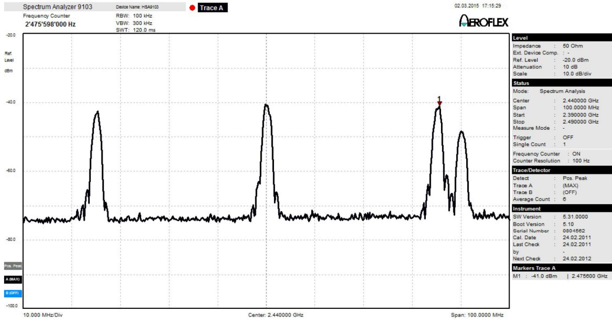
Figure 4-3. Low-Middle-High signals
