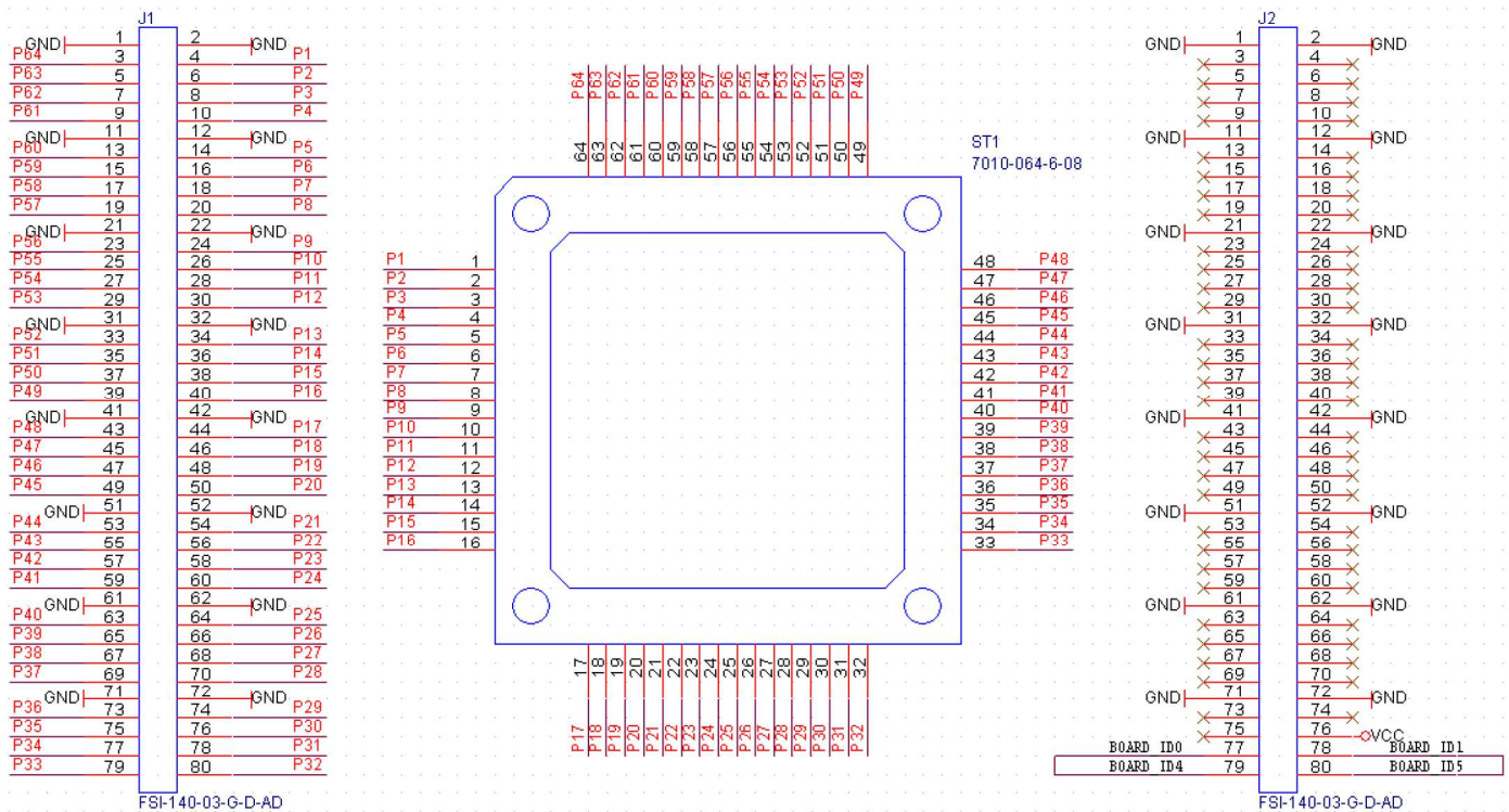
Figure 5-1. Schema capture of socket card.
