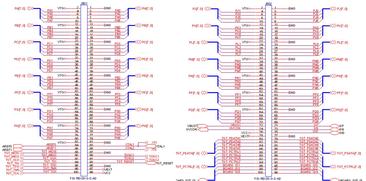
Figure 1-5. STK600 socket connectors' pinout.
