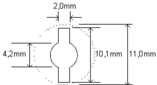
Figure 1-3. Clip hole dimensions.
