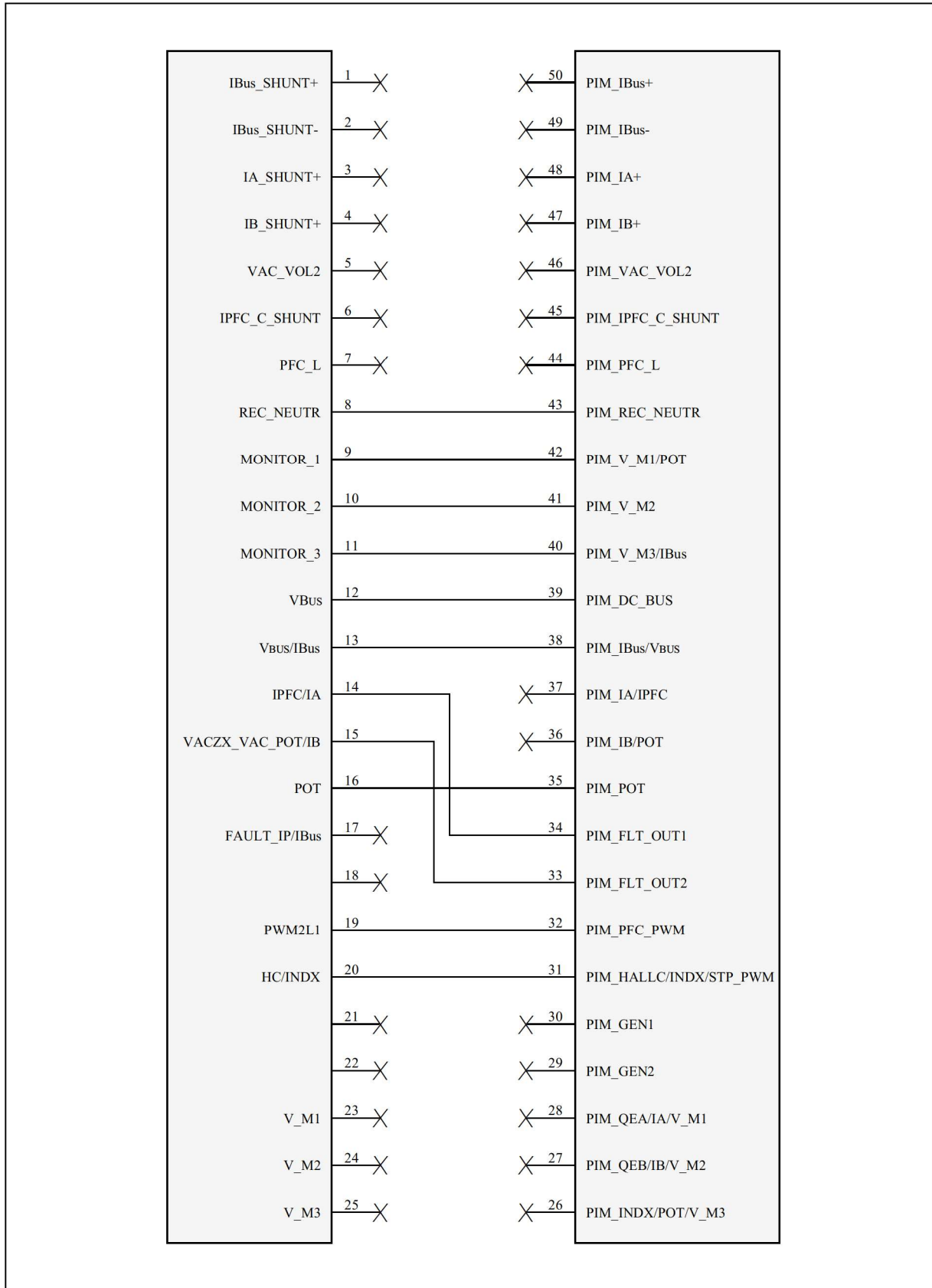
FIGURE A-15: PFC – EXT OP AMP CONFIGURATION BOARD SCHEMATIC
