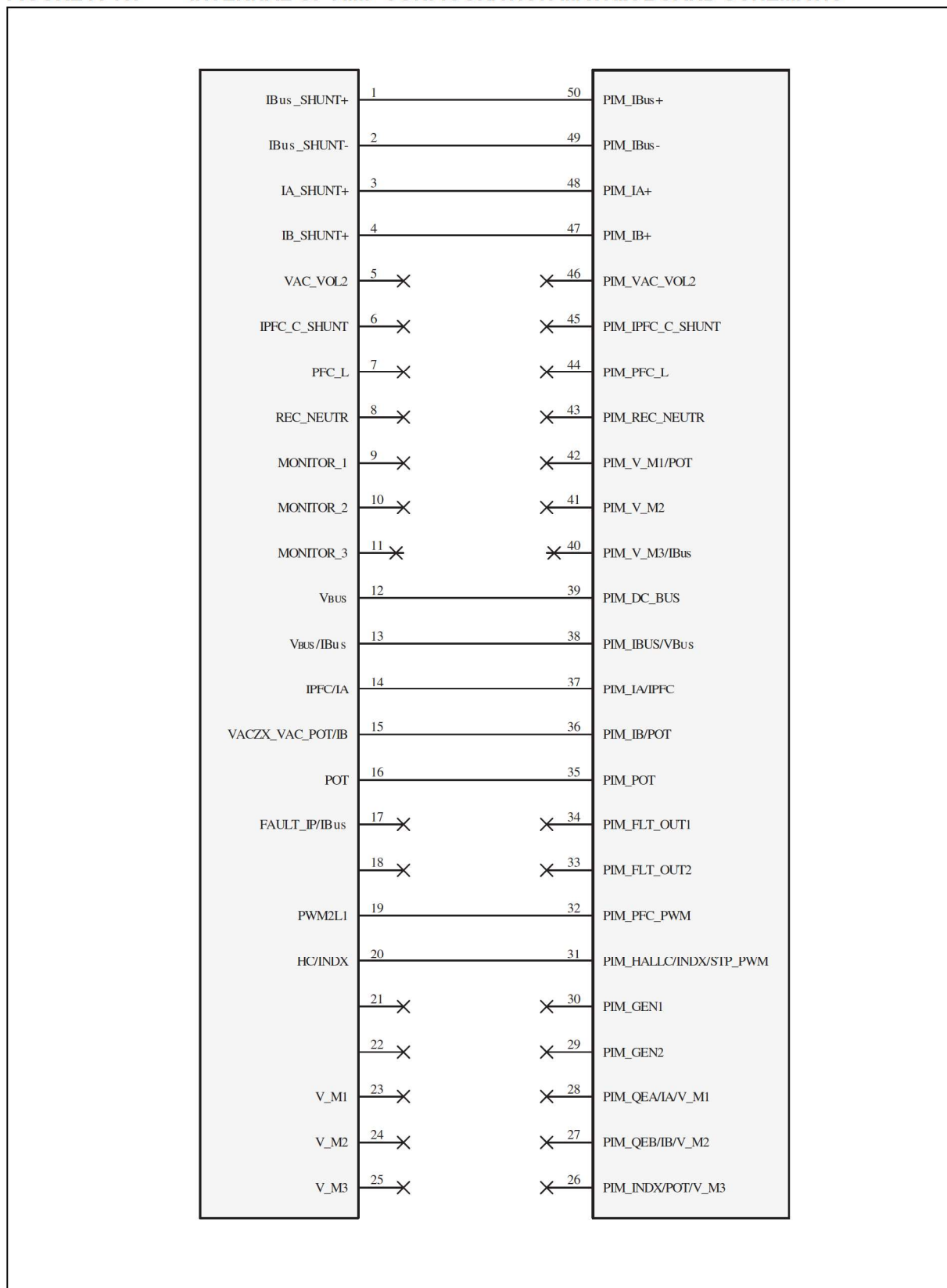
FIGURE A-13: INTERNAL OP AMP CONFIGURATION MATRIX BOARD SCHEMATIC
