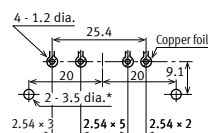
Mounting hole location (Copper-side view)
