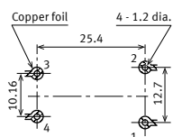
Mounting hole location (Copper-side view)
