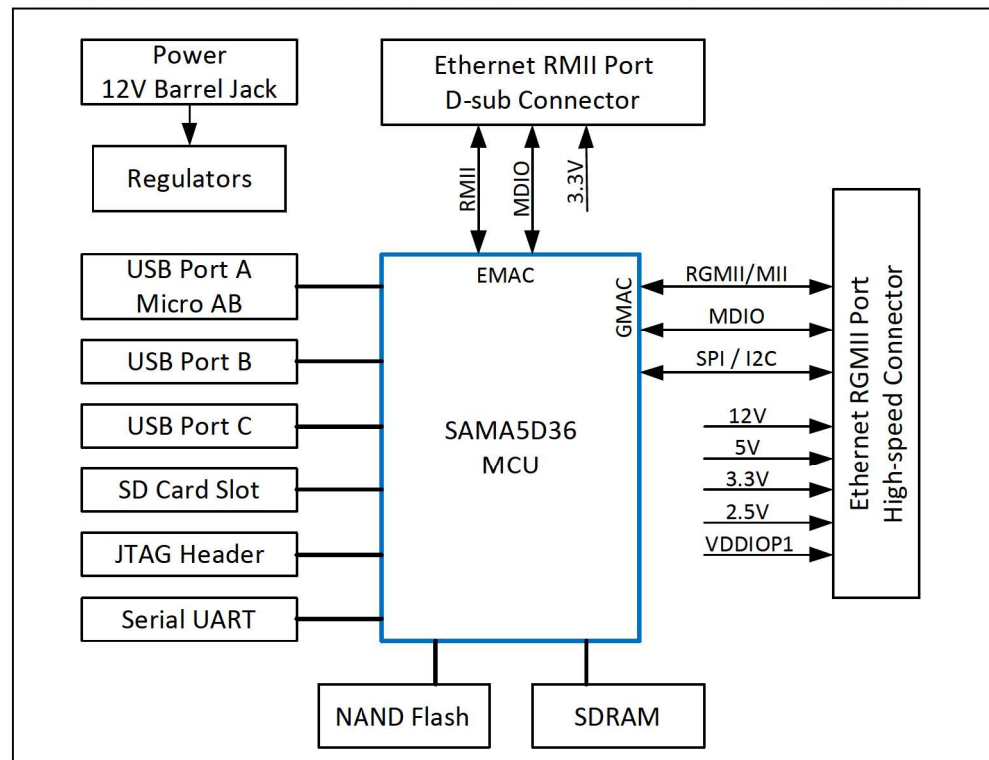
FIGURE 1-1: SAMA5D3 EDS BOARD FUNCTIONAL BLOCK DIAGRAM
