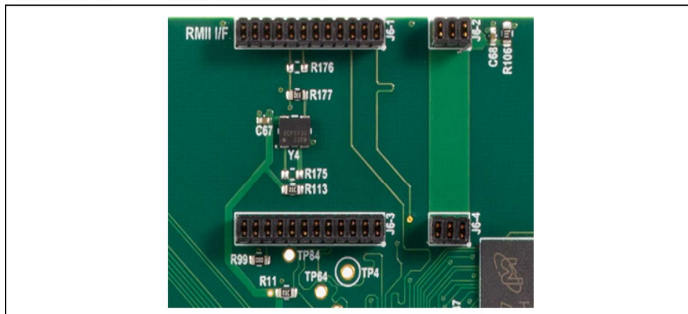
FIGURE 3-4: RMII CONNECTOR
