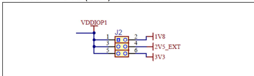
FIGURE 3-3: VDDIP (VARIO) VOLTAGE SELECT
