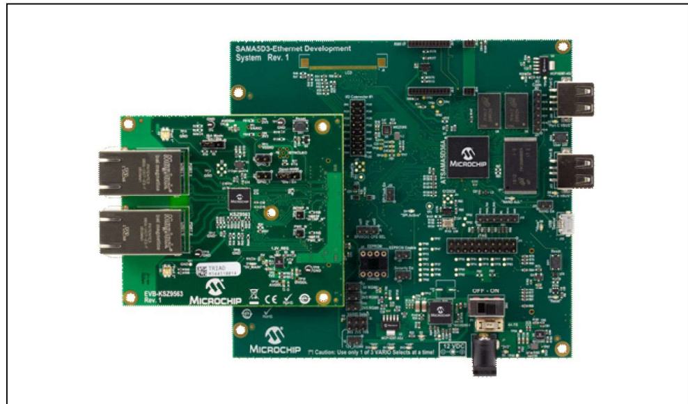
FIGURE 2-1: SAMA5D3 EDS CONNECTED TO THE EVB-KSZ9563
