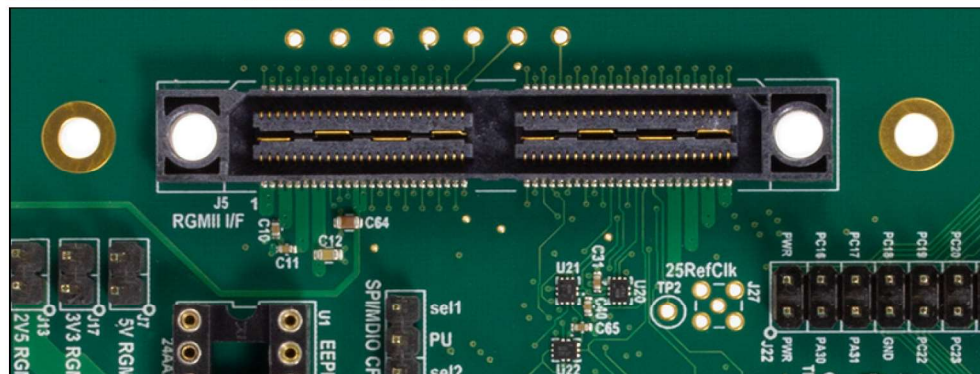
FIGURE 3-2: RGMII CONNECTOR
