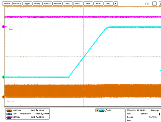
Figure 24. VOUT transition (Vin = VCC = 24 V, Vout = 0x64 (5 V) to 0xF1 (20 V), CC = 0x1F, load = 500 mA, F sw = 500 kHz)
