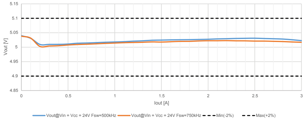
Figure 8. V_{OUT} vs. load ( V_{in} = V_{CC} = 24\text{ V} , V_{out} = 0x64 (5\text{ V}) , CC = 0x1F )
