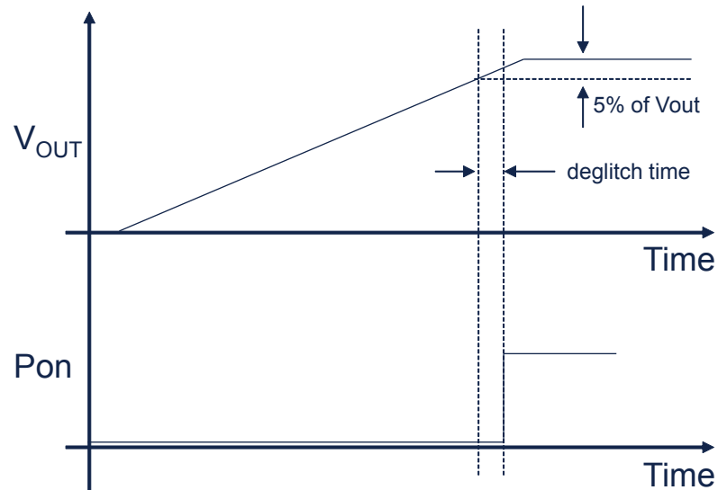
Figure 33. Deglitch time
