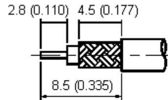
Stripping Dimension
