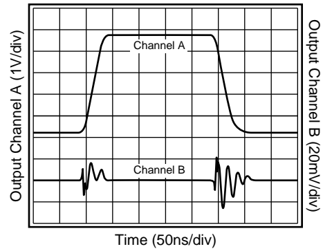
Figure 8: Pulsed crosstalk
