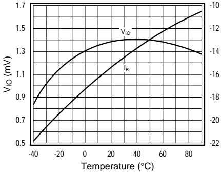
I_B , V_{IO} , vs. Temperature
