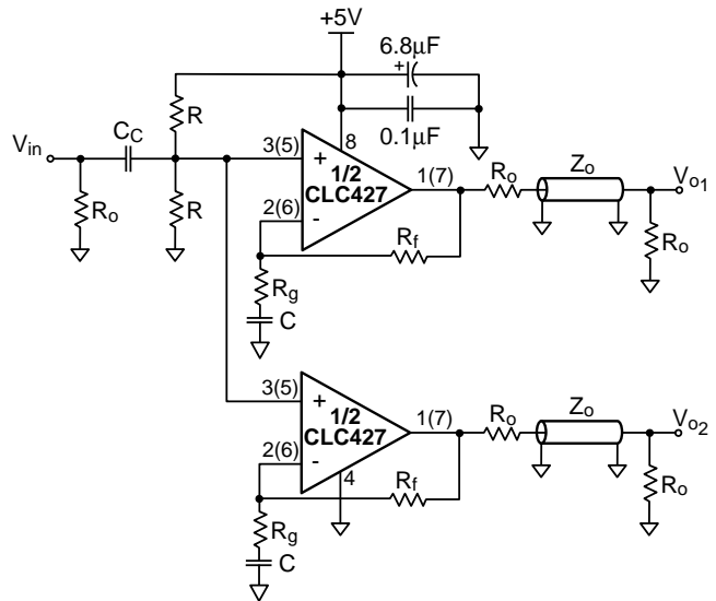
Figure 11: Distribution Amplifier
