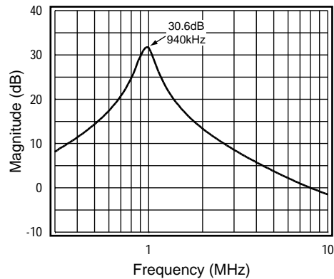
Figure 10: Bandpass Response
