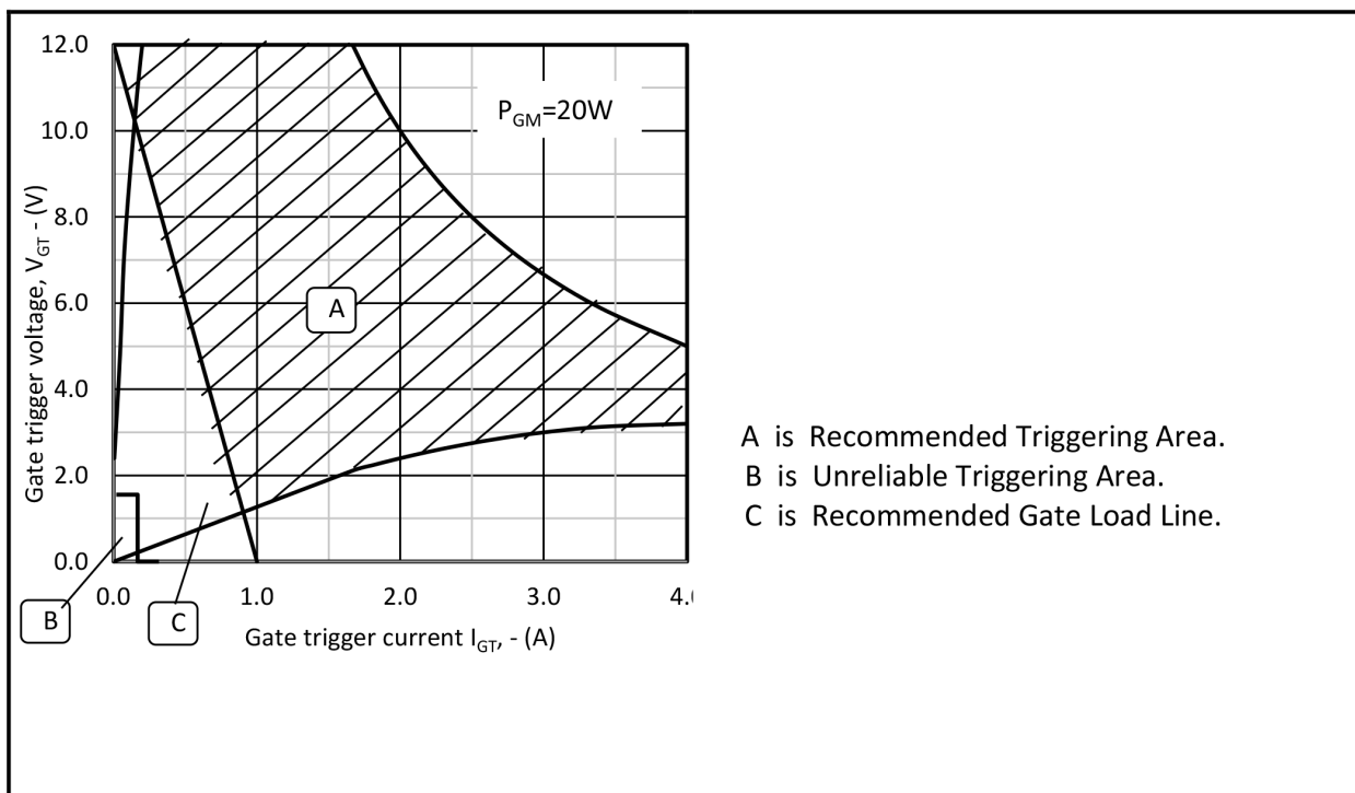
Fig.13 Gate characteristics
