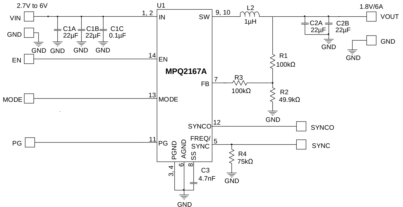
Figure 5: V_{OUT} = 1.8V , I_{OUT} = 6A Application Circuit
