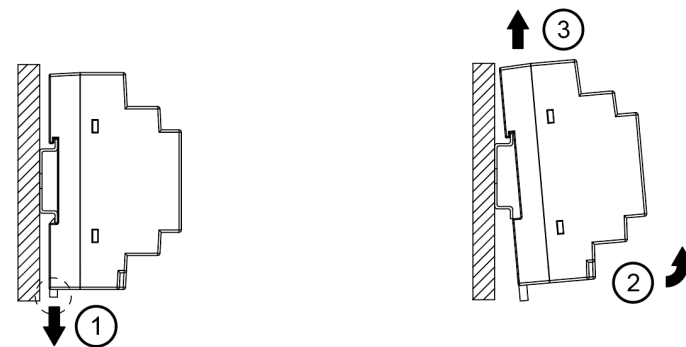
Fig. 2.2 Dismounting
