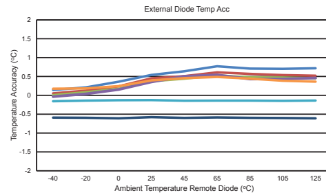
Figure 2-2. Temperature Accuracy vs. Remote Diode Temperature, V_{DD} = 1.8V
