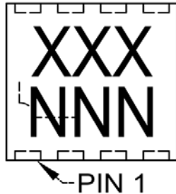
8-Lead WDFN (2 x 2 mm)
