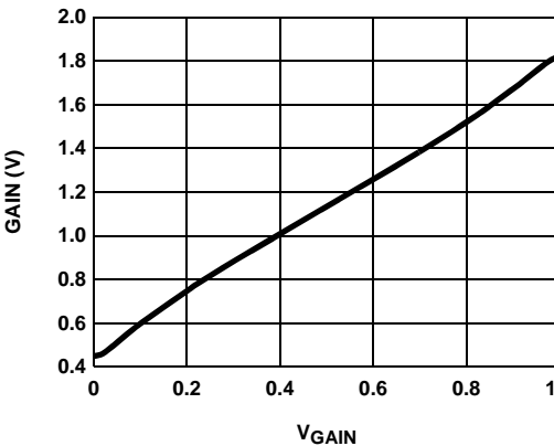
FIGURE 12. VARIATION OF GAIN WITH GAIN CONTROL VOLTAGE
