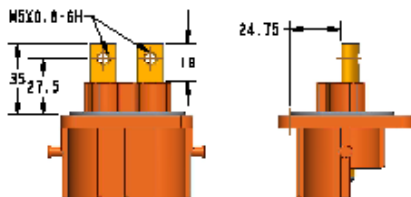
Busbar Type 1
