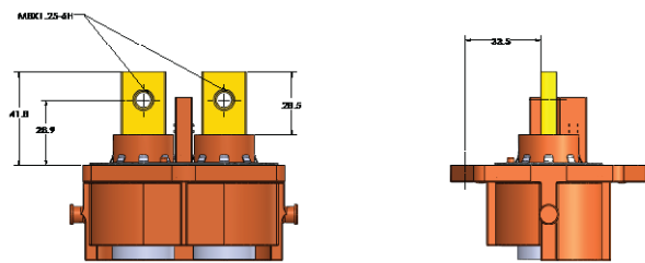
Busbar Type 1
