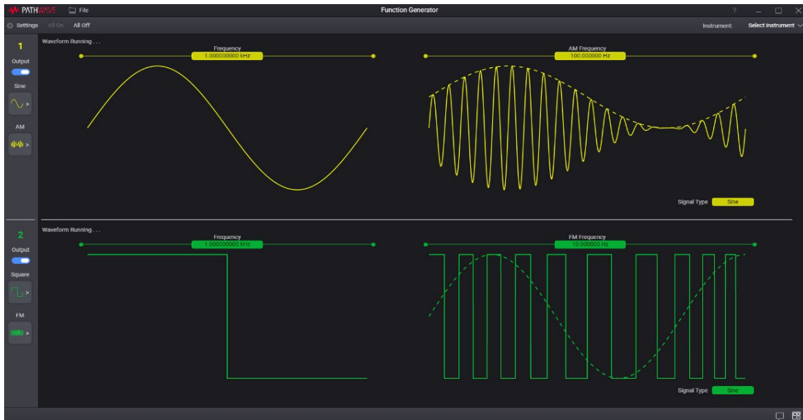
Figure 6. Setting the modulation waveform
