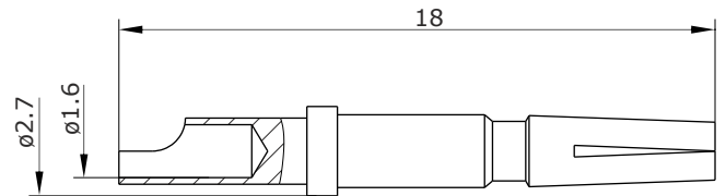
Main Dimensions contact socket
