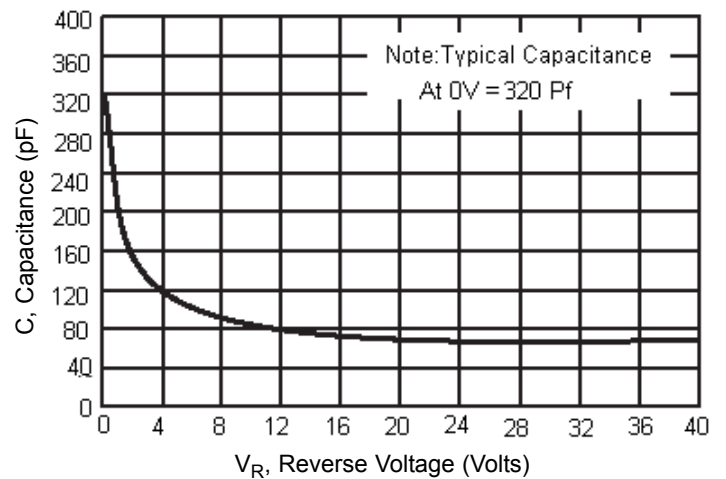
Typical Capacitance
