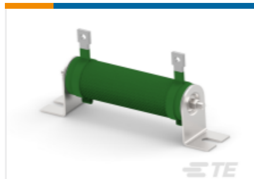
TE Part #2-1879450-2 Wirewound Resistor: Mineral, 2.5 Kw
