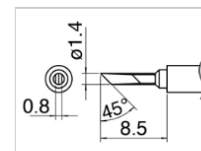
T30-KN Shape-KN N 2 Nozzle assembly B (C5039)*
