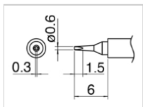
T30-D06 Shape-0.6D N 2 Nozzle assembly A (C5038)*
