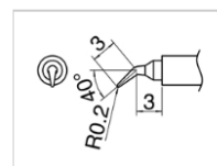
T30-J Shape-J N 2 Nozzle assembly C (C5040)*
