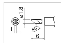
T30-KU Shape-KU N 2 Nozzle assembly A (C5038)*
