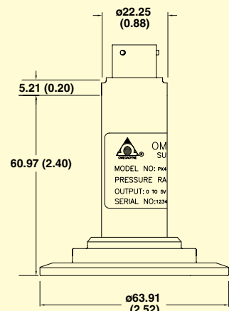
PX429S20 2" flange
