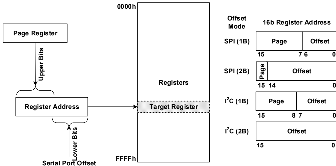
Figure 15. Register Addressing Modes Using Serial Port
