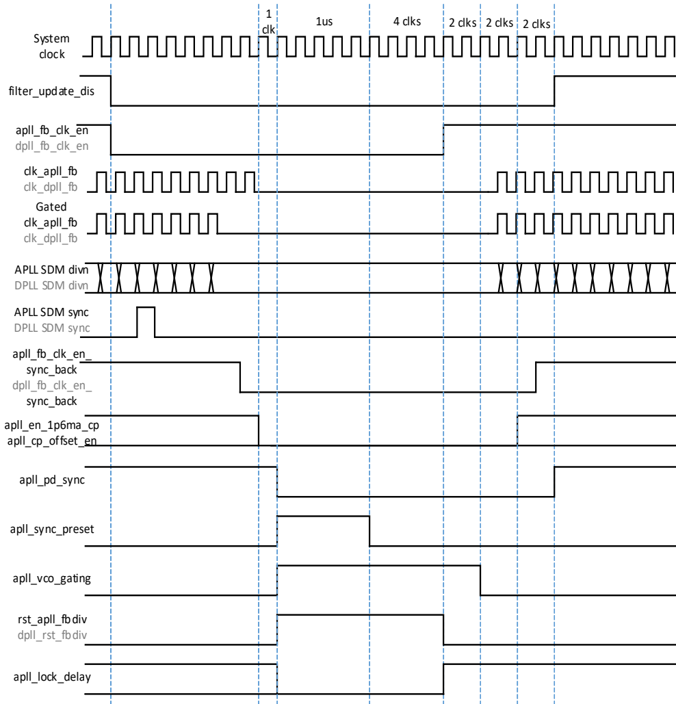
Figure 18. Divider Synchronization Procedure
