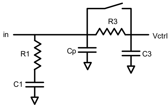
Figure 14. APLL LPF Topology
