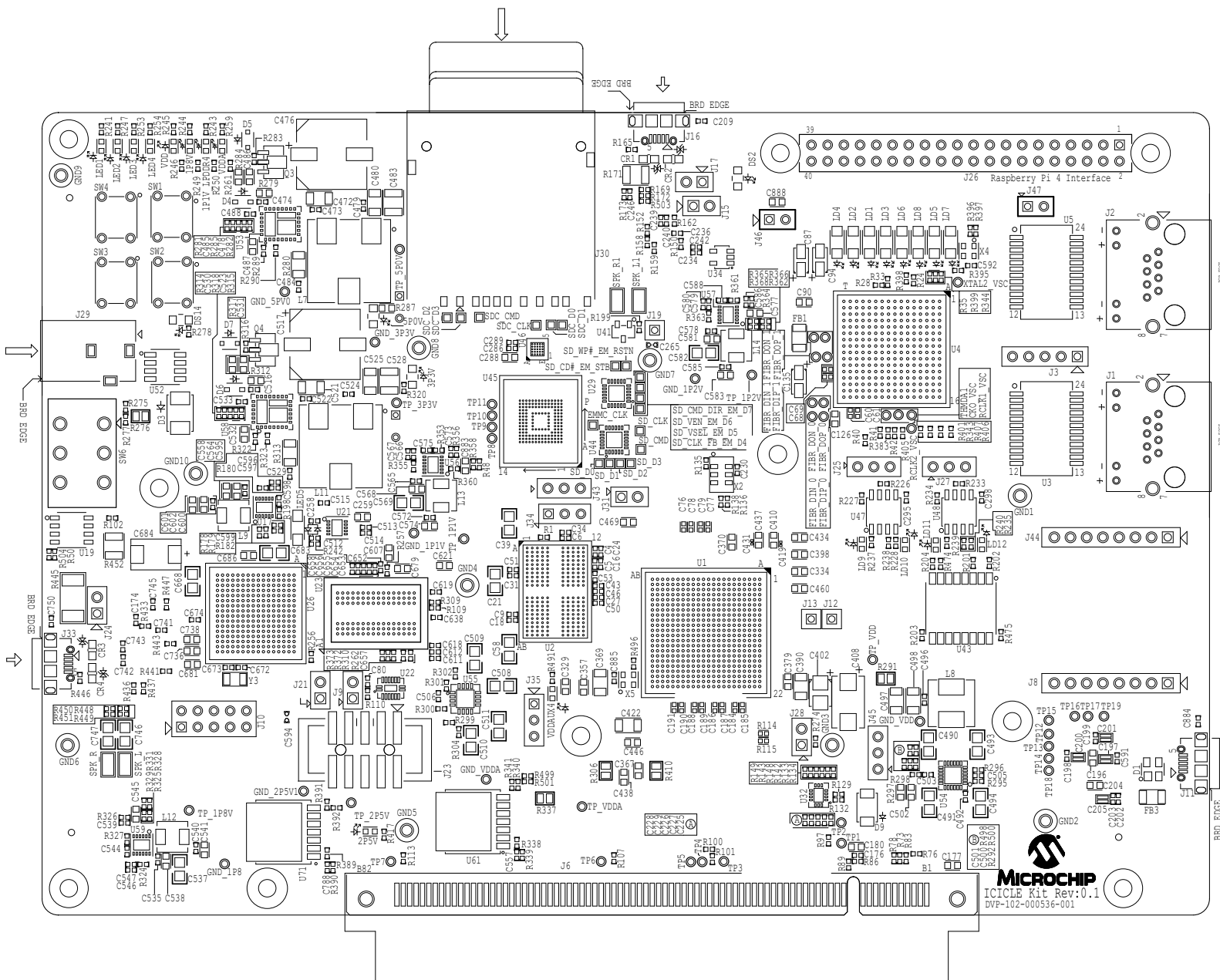
Figure 5-1. Silkscreen Top View
