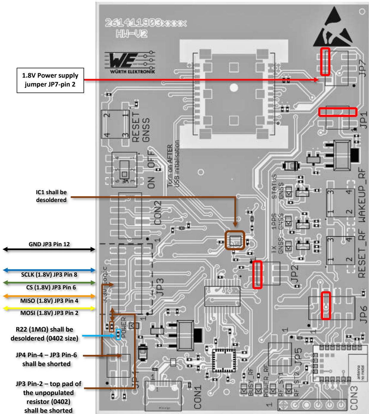
Figure 18: SPI modifications on evaluation board plan (see also real image in Figure 19)
