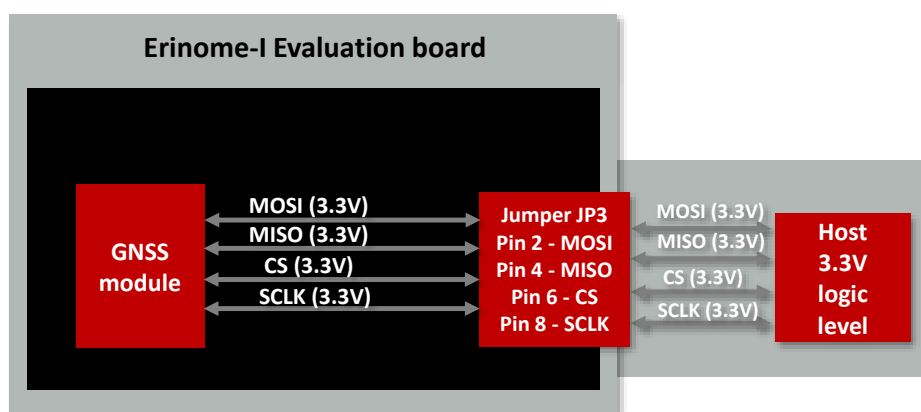
Figure 17: SPI Hardware setup
