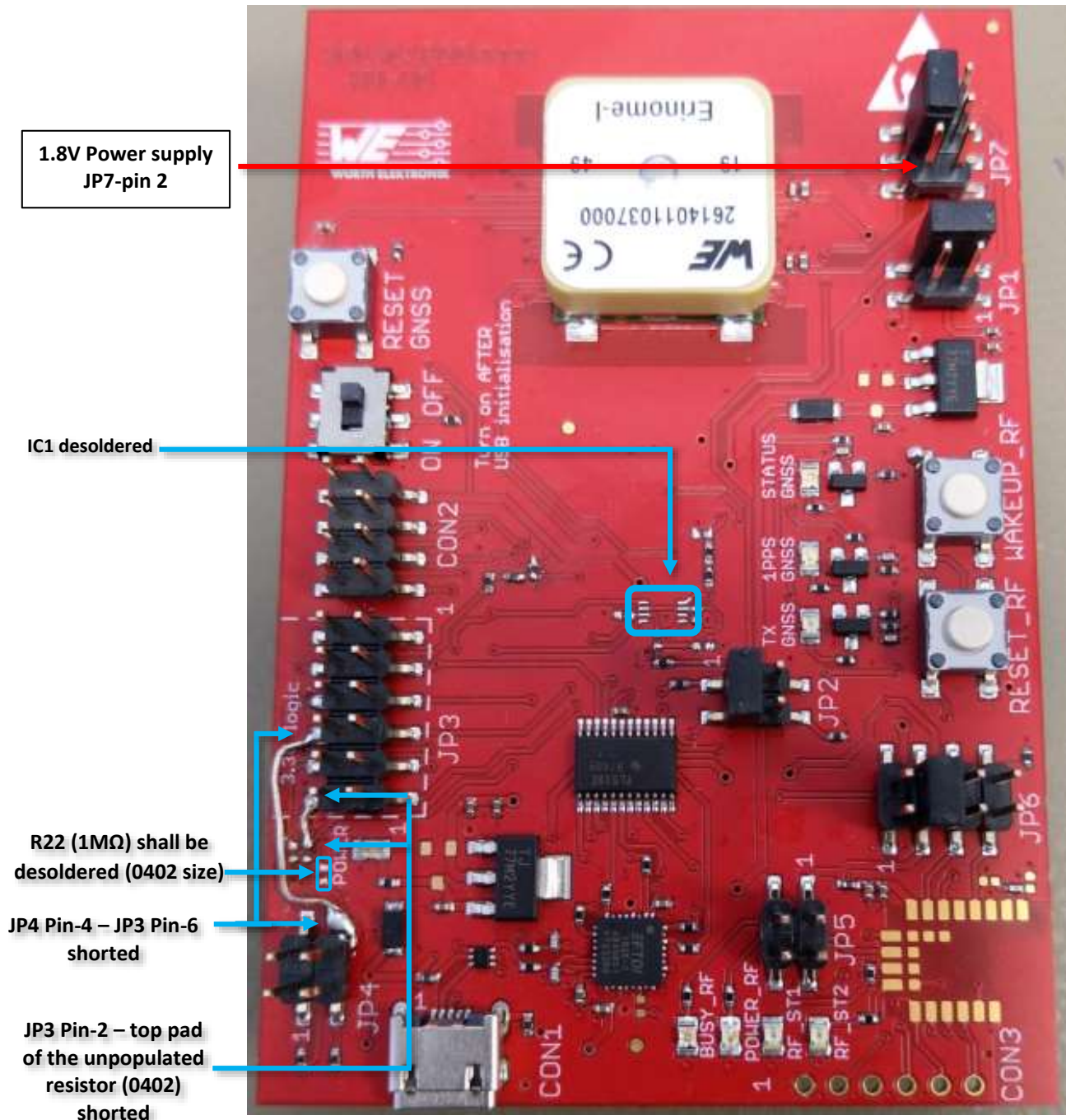
Figure 19: Modified evaluation board for SPI communication
