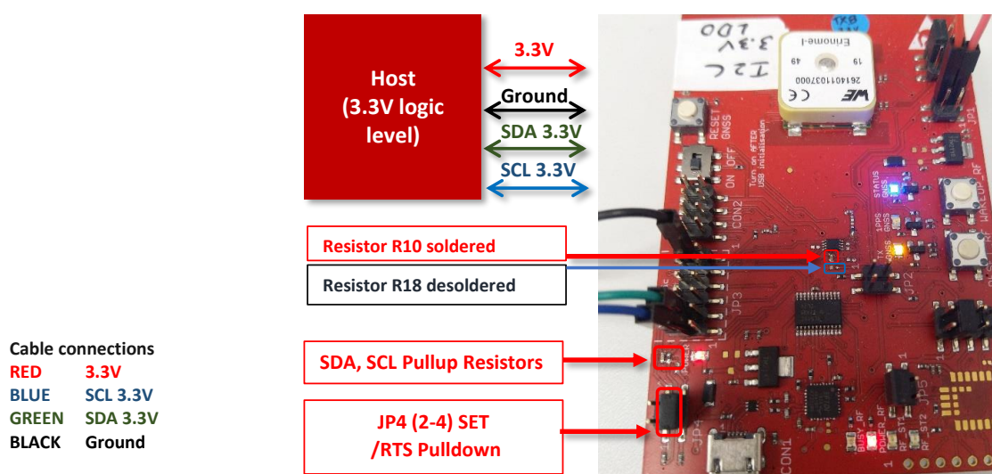
Figure 16: 3.3V - Erinome-I evaluation board connection to 3.3V Host
