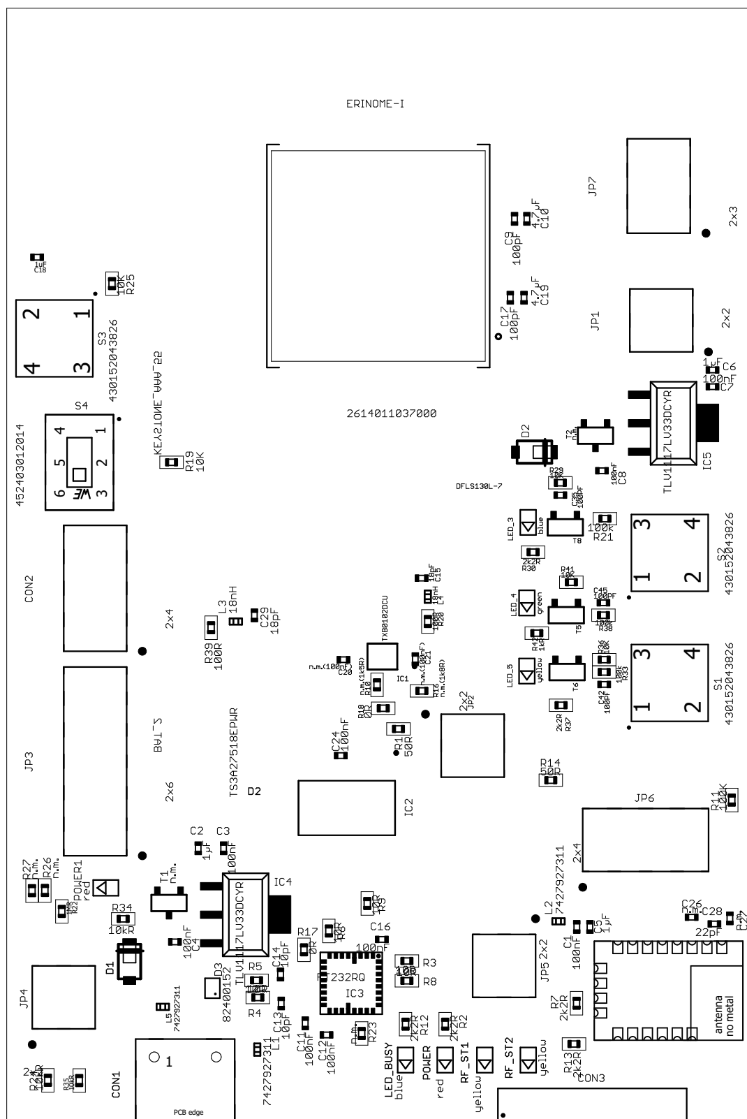
Figure 10: Assembly diagram
