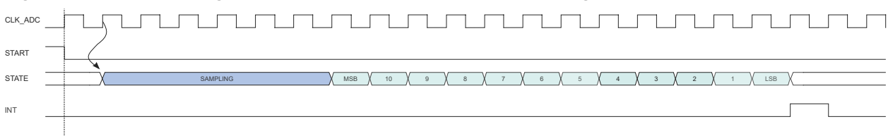
Figure 13-206. ADC Timing for One Conversion with Increased Sampling Time, 12-bit
