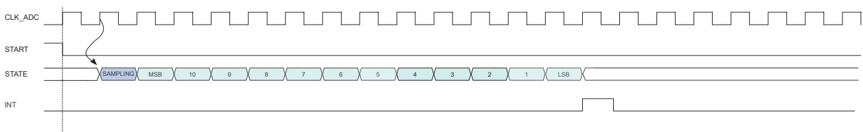
Figure 13-205. ADC Timing for One Conversion in 12-bit Resolution
