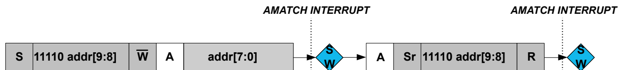
Figure 13-118. 10-bit Addressing
