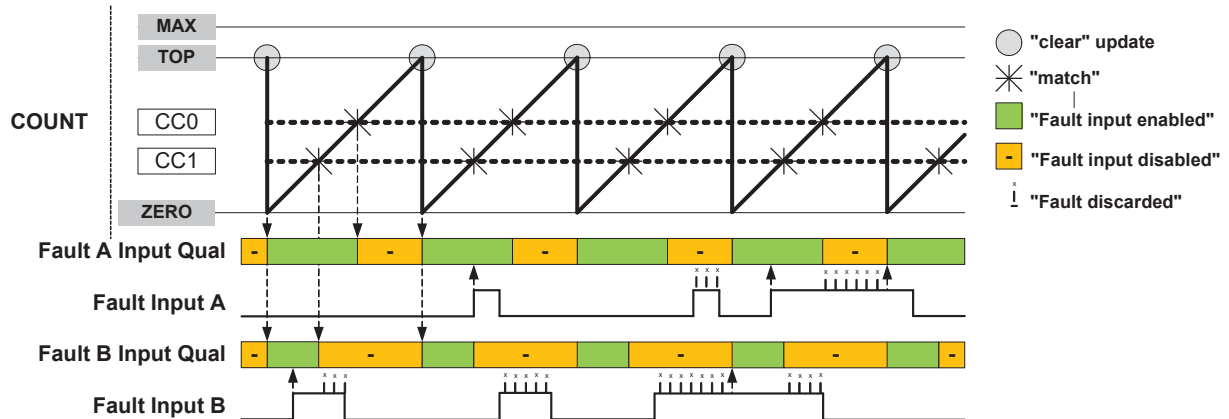
Figure 13-160. Fault Qualification in RAMP2 Operation with Inverted Polarity
