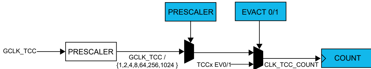
Figure 13-138. Prescaler
