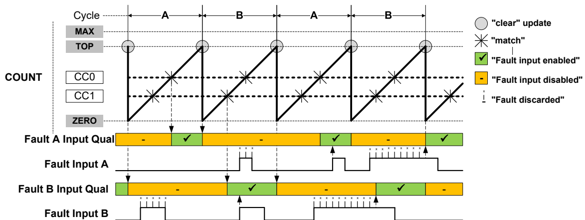
Figure 13-160. Fault Qualification in RAMP2 Operation with Inverted Polarity
