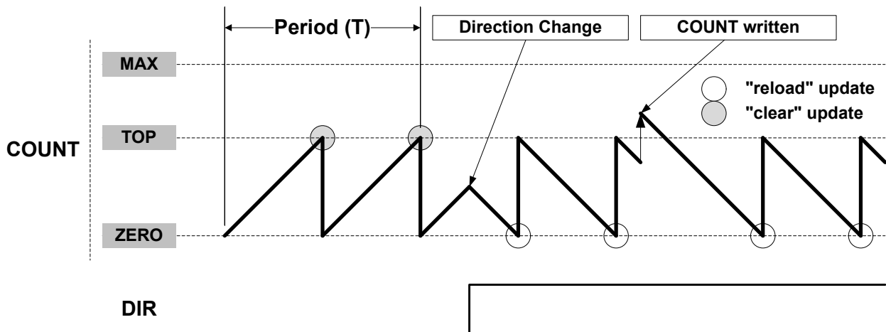
Figure 13-123. Counter Operation
