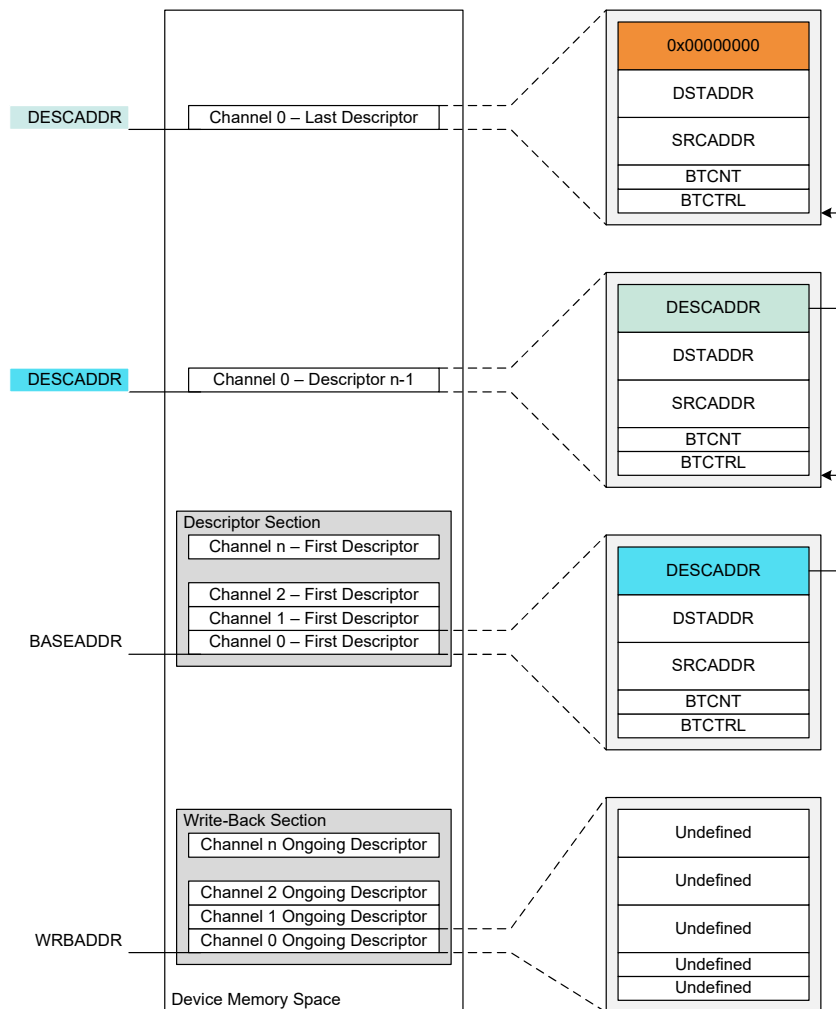
Figure 13-49. Memory Sections
