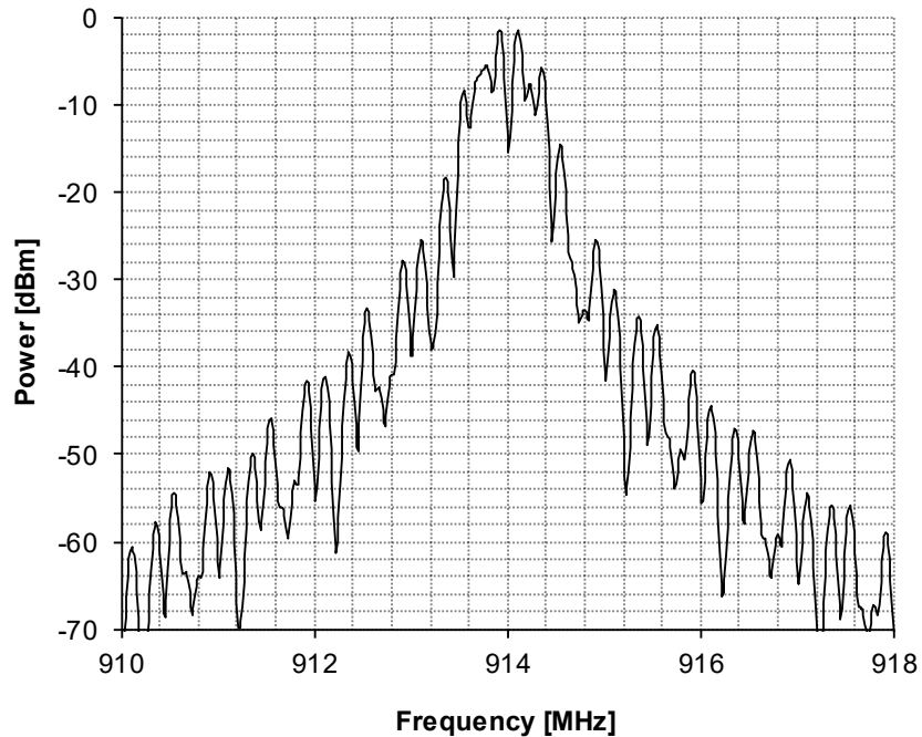
Figure 14-46. Spectrum of OQPSK-RC-250
