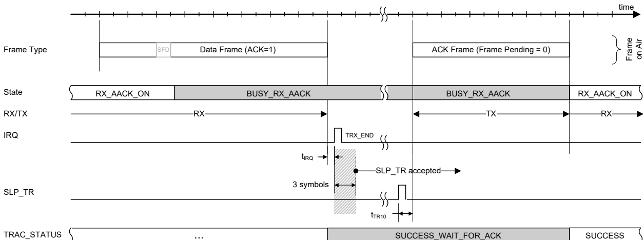
Figure 14-28. Timing Example of an RX_AACK Transaction for Slotted Operation
