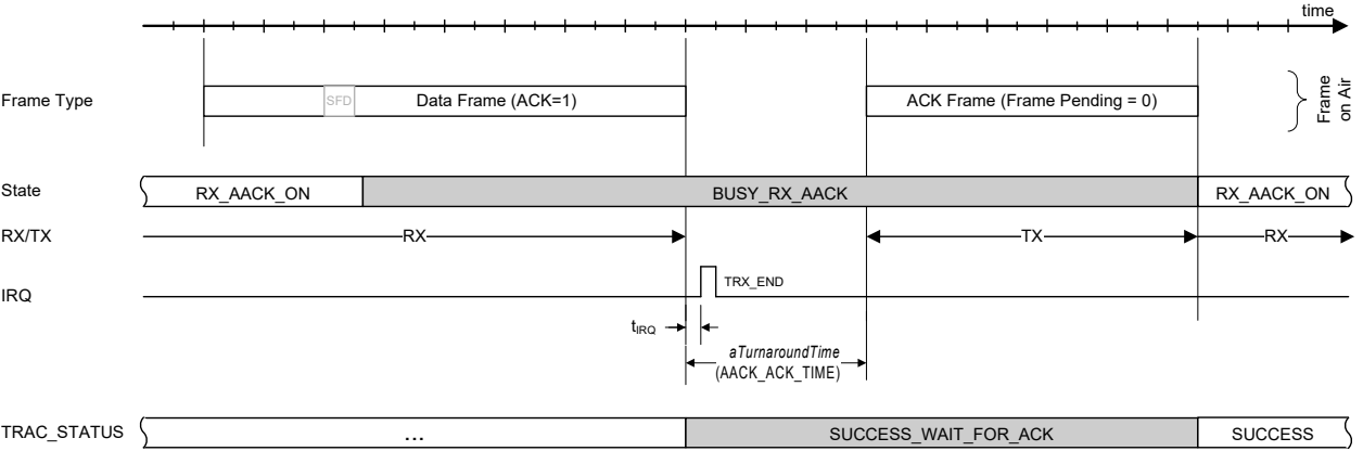
Figure 14-29. Timing Example of an RX_AACK Transaction
