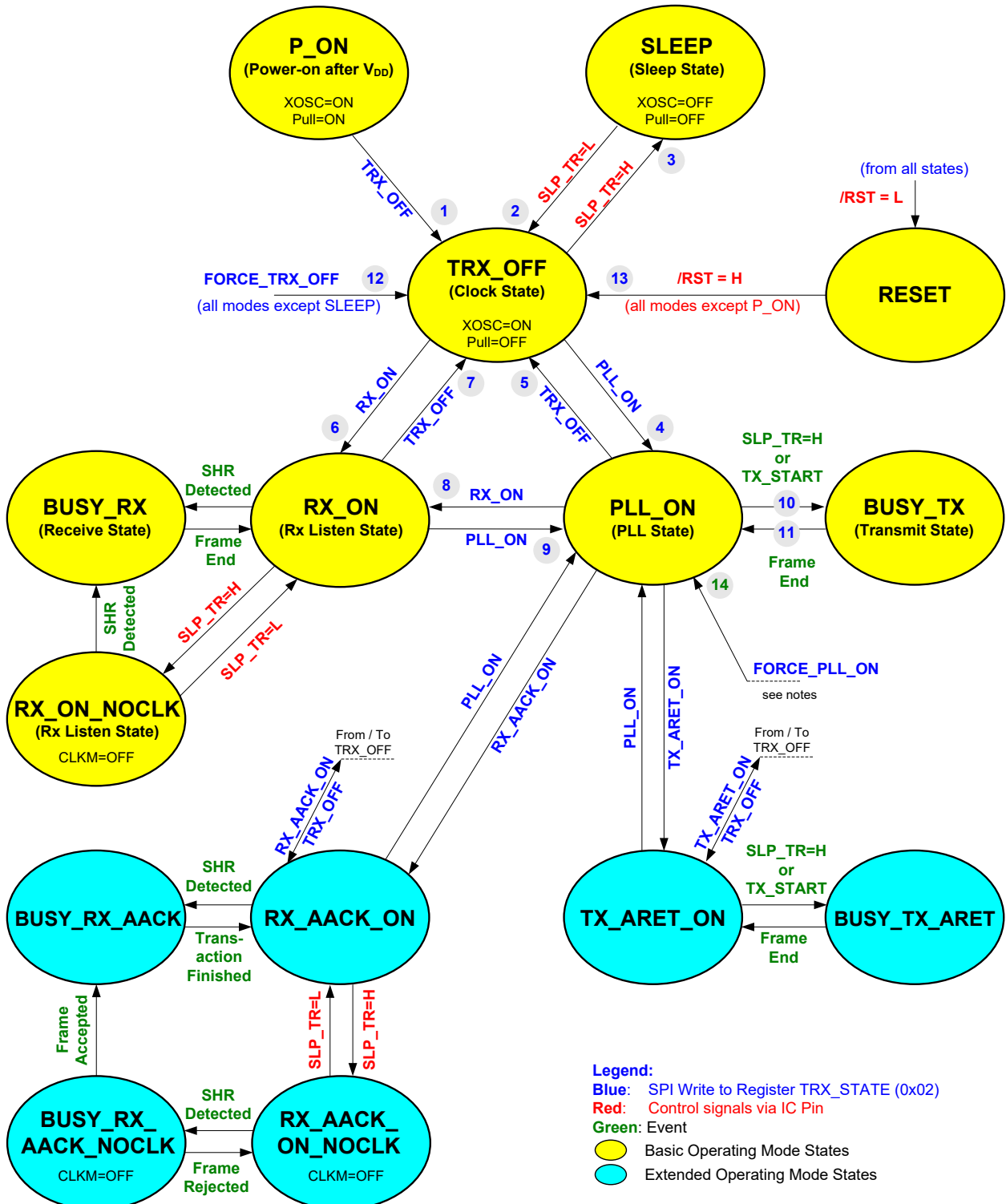
Figure 14-26. Extended Operating Mode State Diagram
