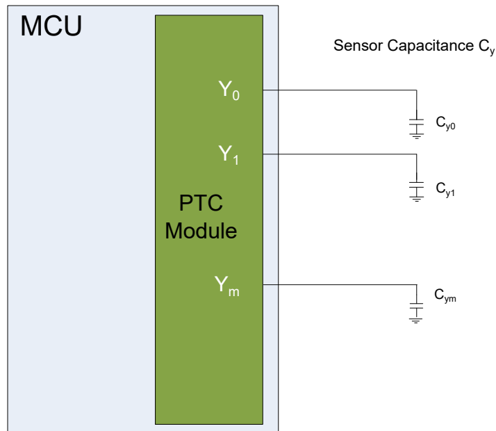
Figure 13-224. Self-capacitance Sensor Arrangement
