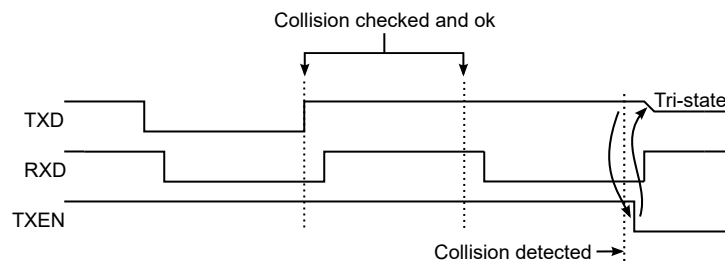
Figure 13-100. Collision Detected
