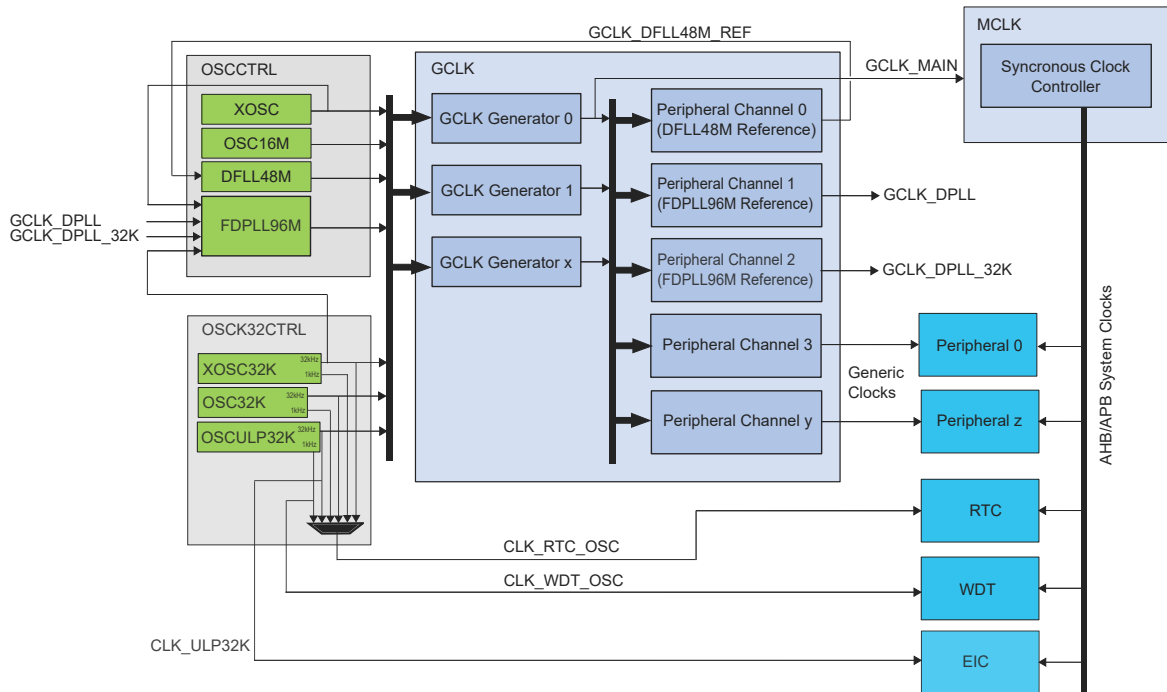
Figure 13-8. Clock Distribution
