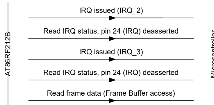
Figure 14-54. Transactions between AT86RF212B and Microcontroller during Receive
