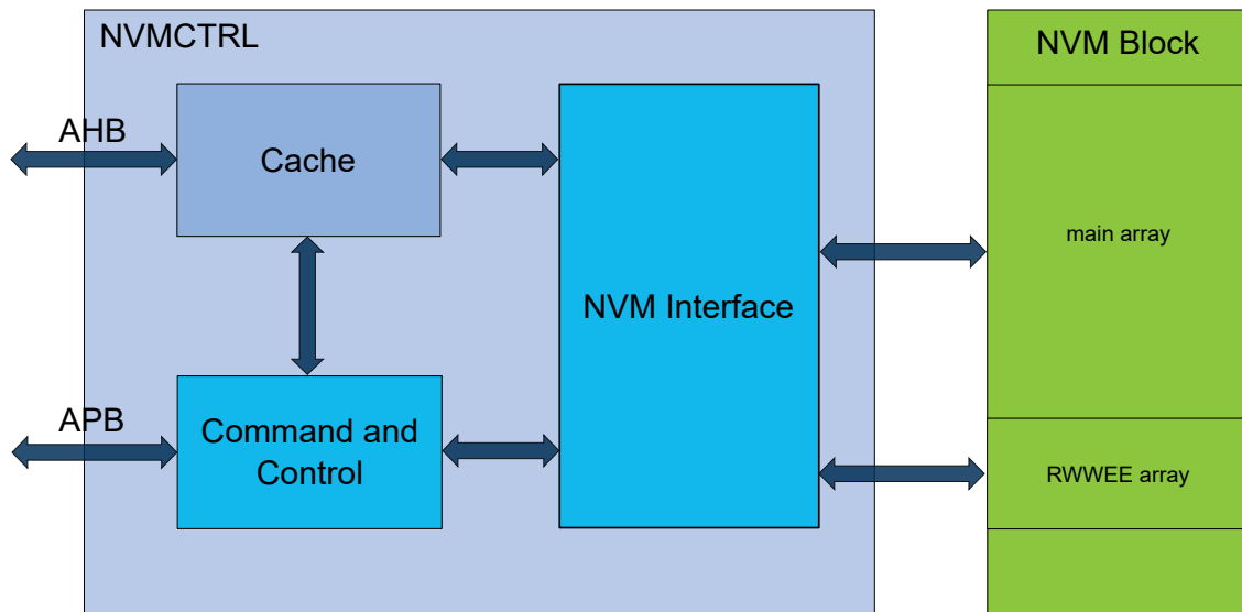
Figure 13-66. Block Diagram
