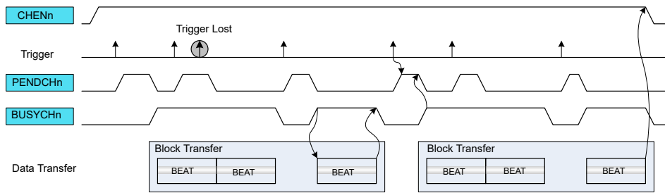
Figure 13-53. Trigger Action and Transfers
