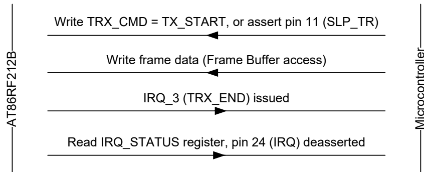
Figure 14-56. Time Optimized Frame Transmit Procedure
