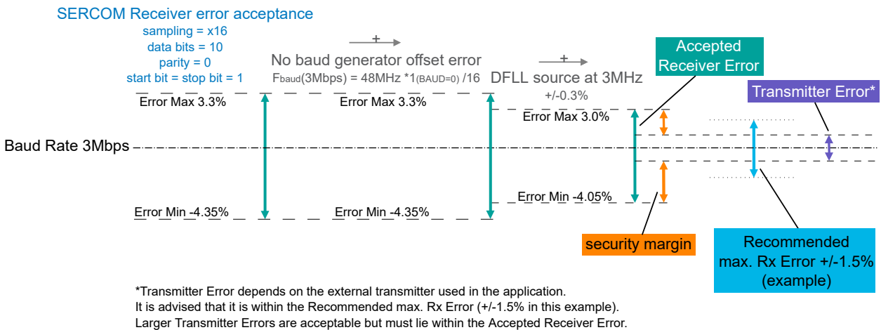
Figure 13-92. USART Rx Error Calculation Example
