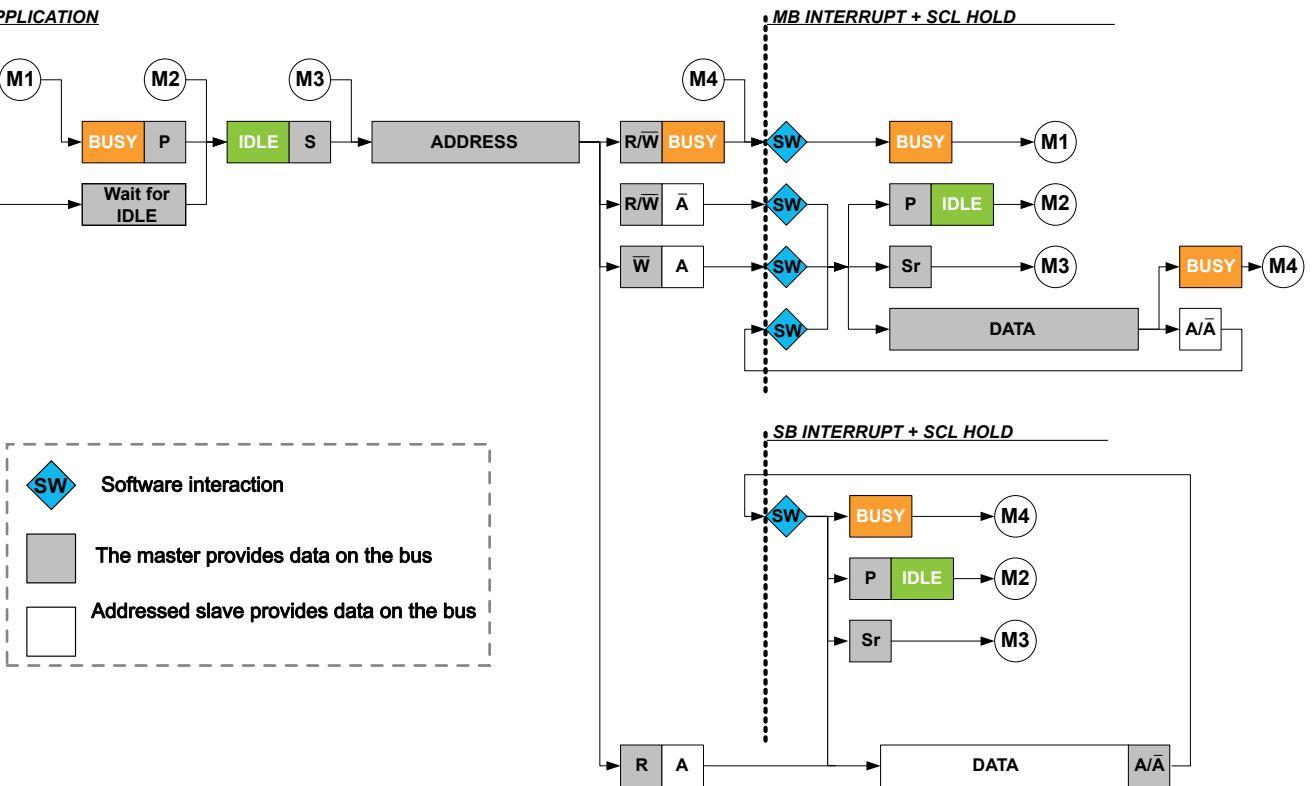
Figure 13-112. I 2 C Master Behavioral Diagram (SCLSM=1)
