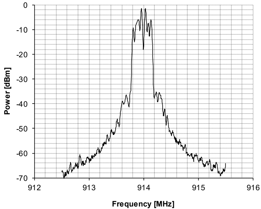
Figure 14-44. Spectrum of OQPSK-RC-100
