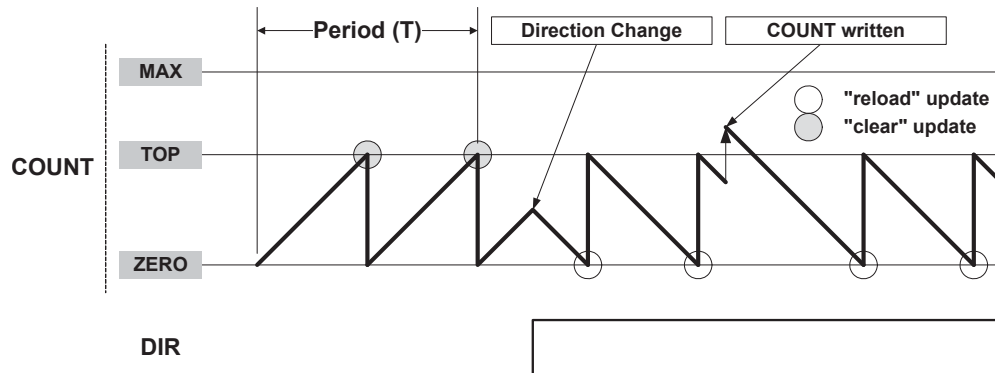
Figure 13-139. Counter Operation
