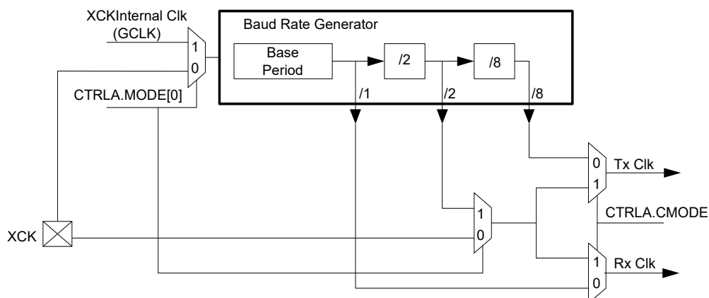
Figure 13-89. Clock Generation
