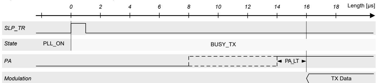
Figure 14-47. TX Power Ramping Example (O-QPSK 250kb/s Mode)
