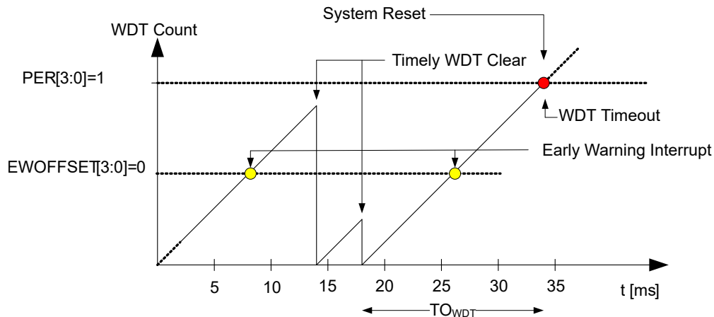
Figure 13-41. Normal-Mode Operation
