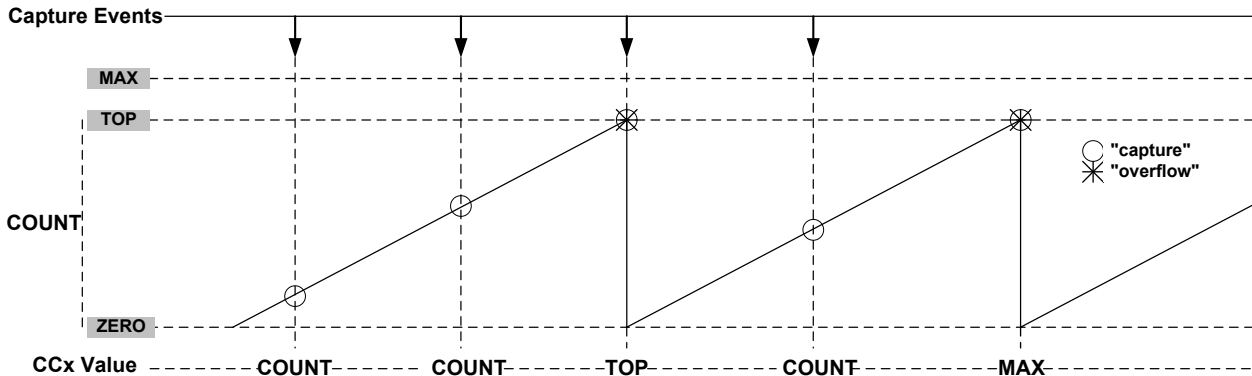
Figure 13-135. Time-Stamp
