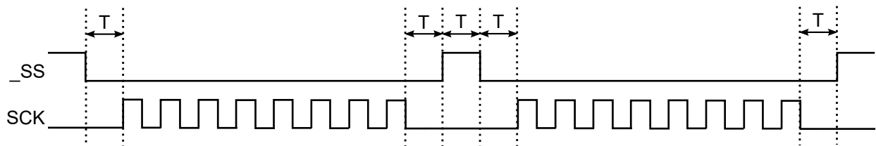
Figure 13-107. Hardware Controlled \overline{SS}
