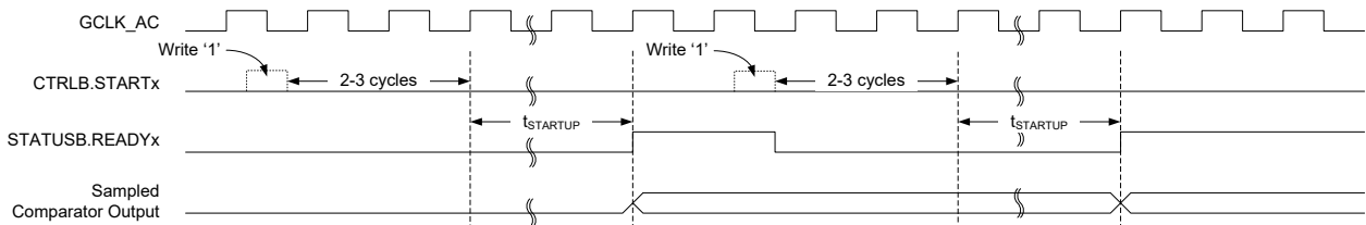
Figure 13-213. Single-Shot Example
