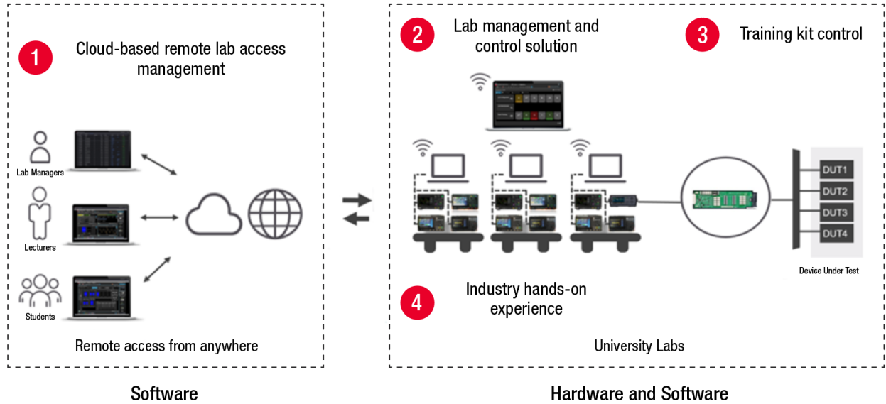
Figure 1. Keysight Industry-ready Remote Access Lab Solution
