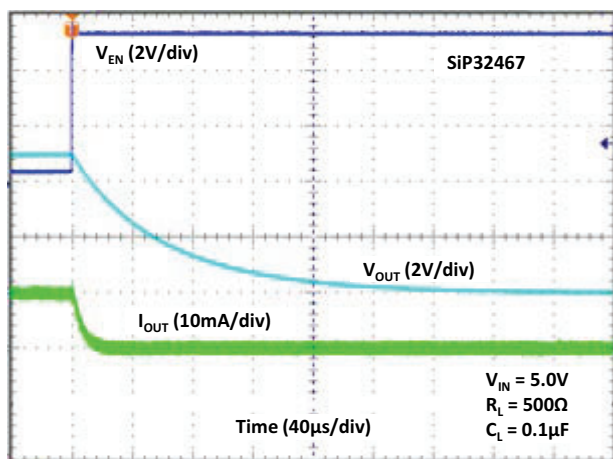
Fig. 30 - Turn-off Time
