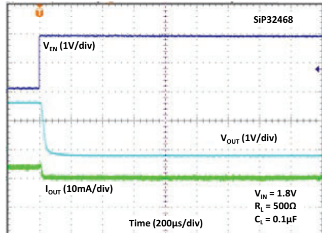
Fig. 33 - Turn-off Time
