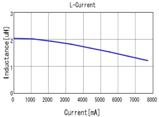
DFE322520FD-2R2M L-Current 20degC
