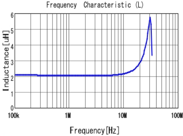
DFE322520FD-2R2M L
