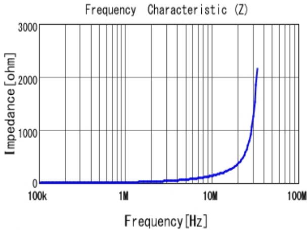
DFE322520FD-2R2M |Z|
