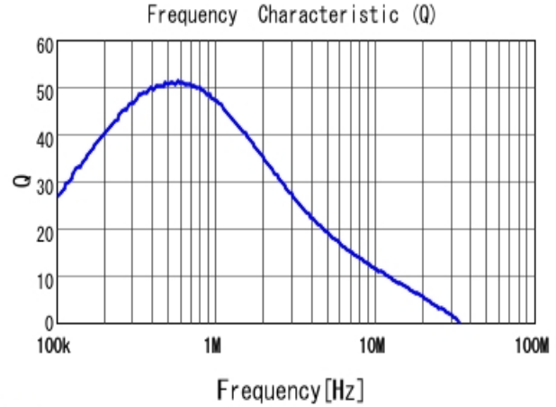
DFE322520FD-2R2M Q
