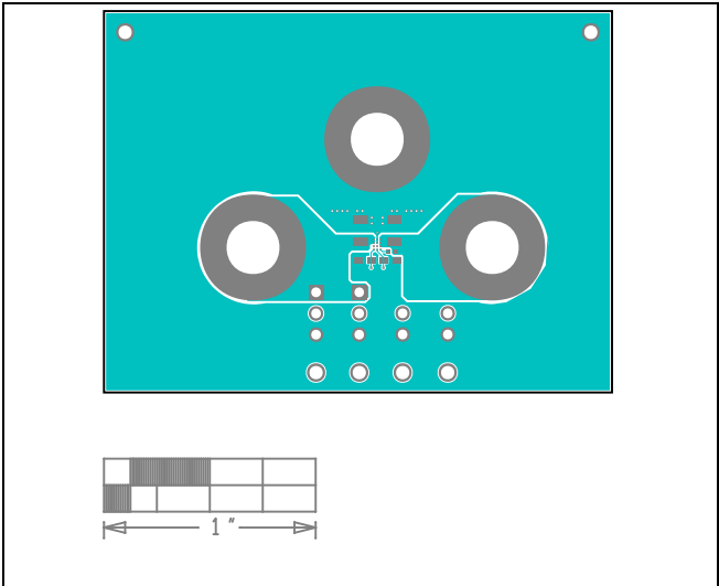
MAX38913A WLP EV Kit PCB Layout—Top
