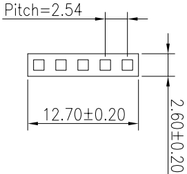
HOUSING
