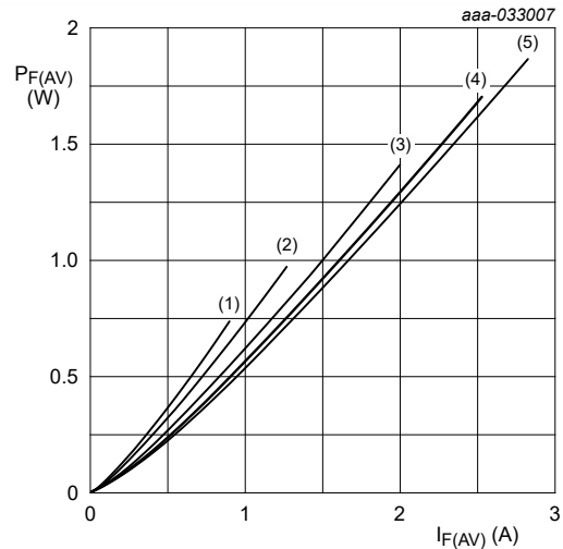
T_j = 100\text{ }^\circ\text{C} (1) \delta = 0.1 (2) \delta = 0.2 (3) \delta = 0.5 (4) \delta = 1 ; DC
