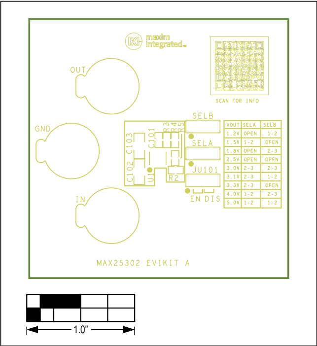
MAX25302 EV Kit—Bottom View
