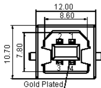
Straight Detail Scale 2 : 1
