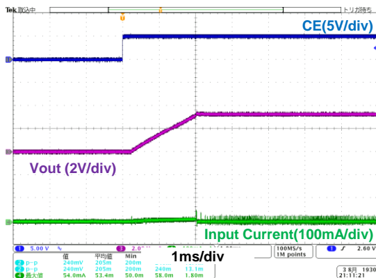
(5-3) Vin = 24V, Iout = 10mA
