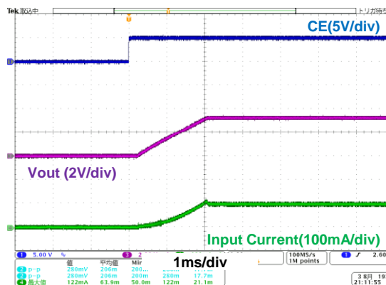
(5-2) Vin = 12V, Iout = 300mA
