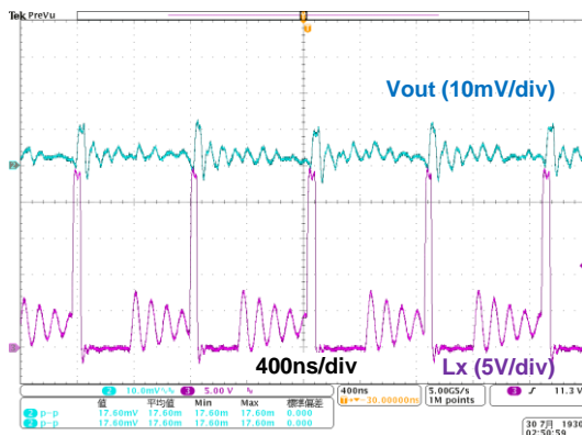
(4-3) Vin = 24V, Iout = 50mA
