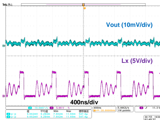
(4-1) Vin = 12V, Iout = 50mA
